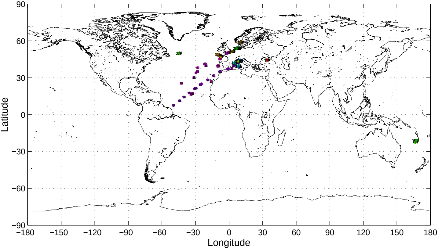
MUD=SIMBADA-2003020400 (ID=1)
