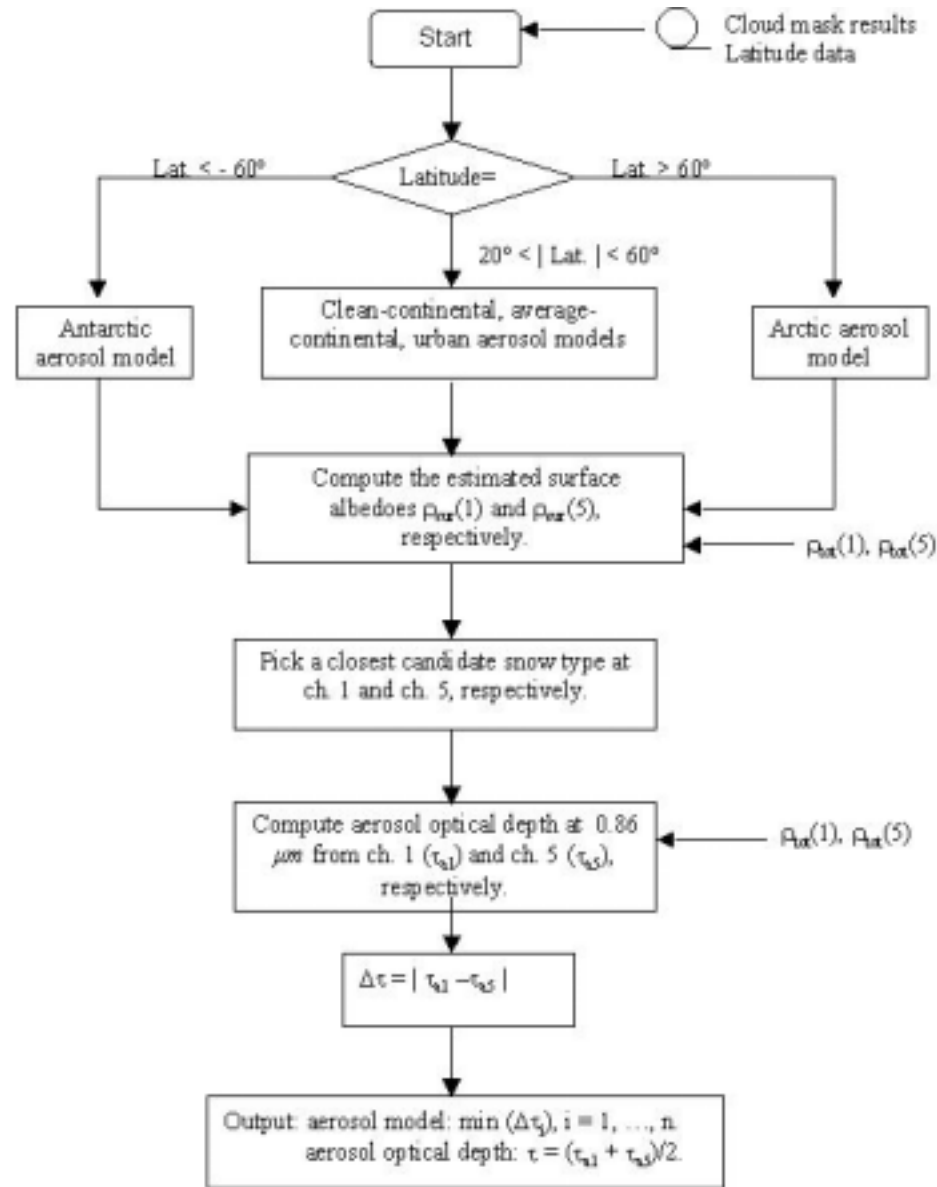
Figure 2.9 Flow chart of aerosol model and aerosol optical depth retrieval. \rho_{toa}(1) and \rho_{toa}(5) are the TOA reflectances of GLI channels 1 ( 0.38 \mu m ) and 5 ( 0.46 \mu m ), respectively. \rho_{sur}(1) and \rho_{sur}(5) are the Lambertian surface albedo values at GLI channels 1 and 5, respectively. The \tau_{a1} and \tau_{a5} are the aerosol optical depth \tau ( 0.86 \mu m ) retrieved from GLI channels 1 and 5, respectively, and n is the total number of candidate aerosol models.
