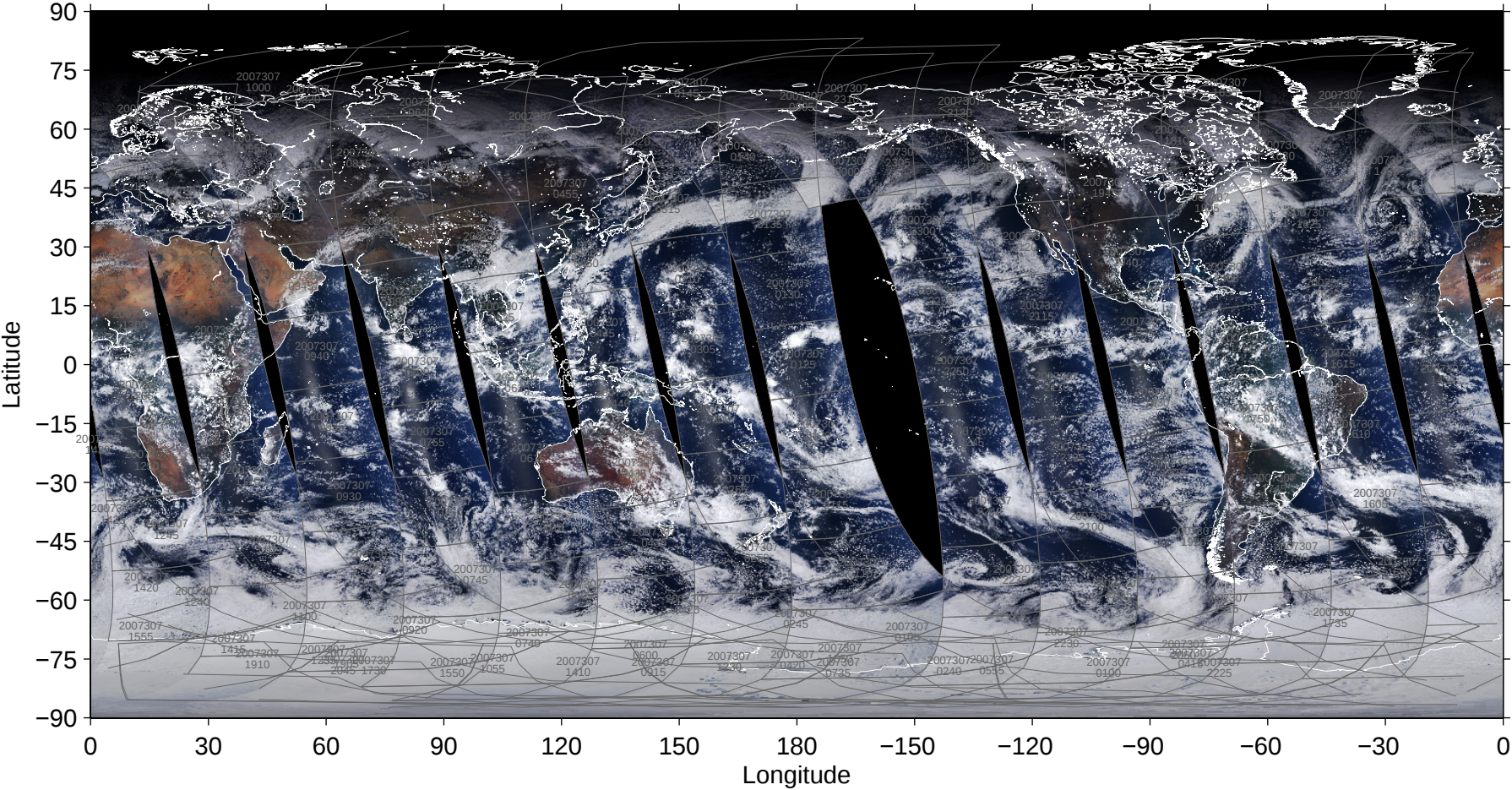
File = MYD02SSH-A2007307-pbin-005.1440-0721, RGB=645, 555, 469nm
