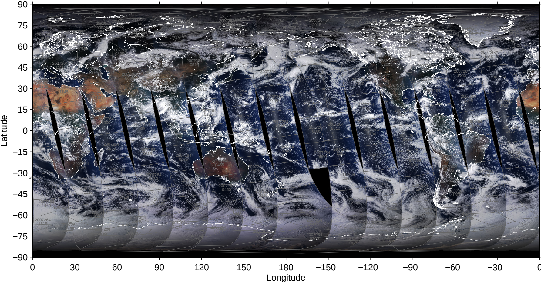
File = 200709/MYD02SSH-A2007264-pbin-005.1440-0721, RGB=645, 555, 469nm
