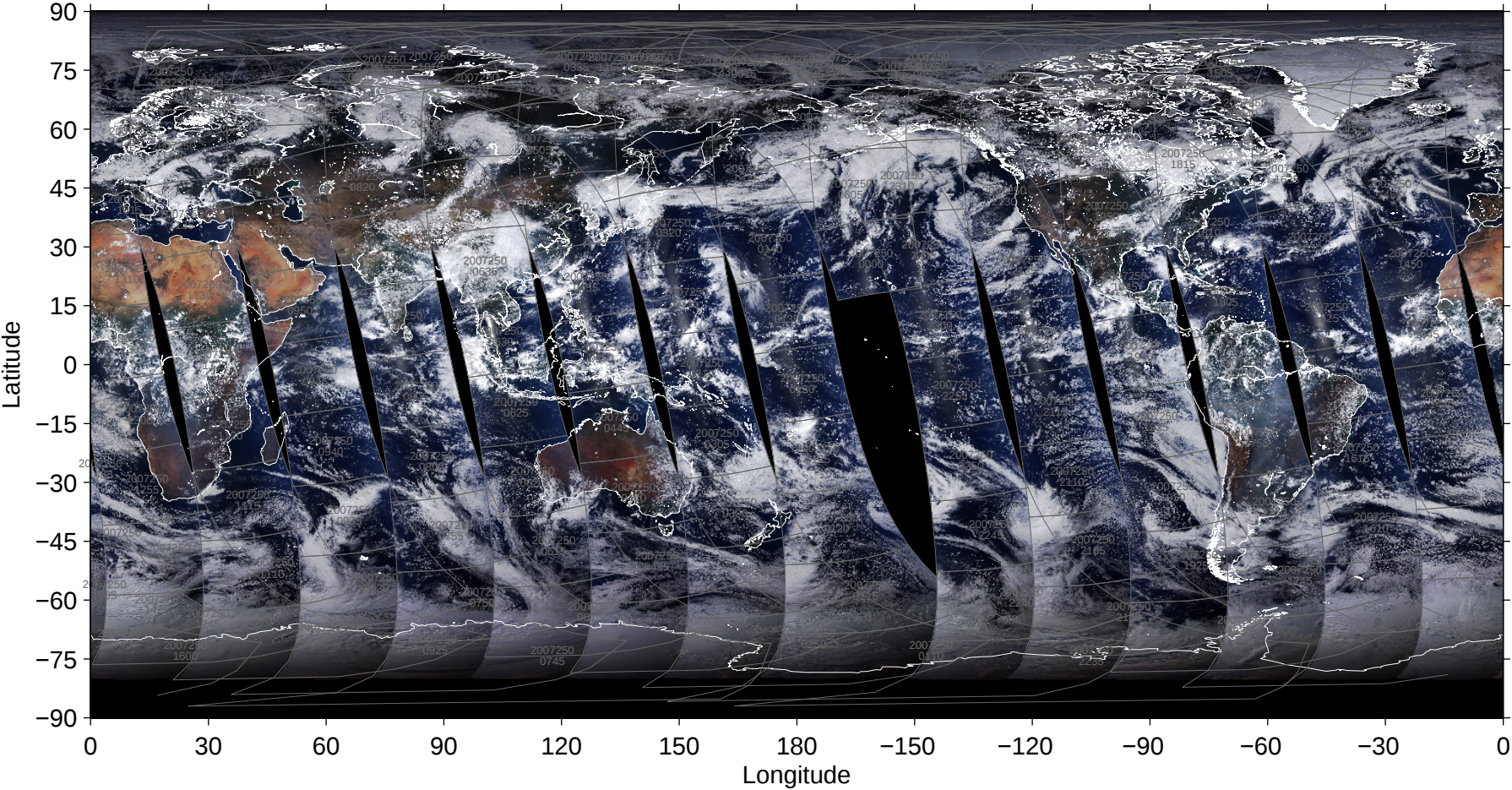
File = 200709/MYD02SSH-A2007250-pbin-005.1440-0721, RGB=645, 555, 469nm
