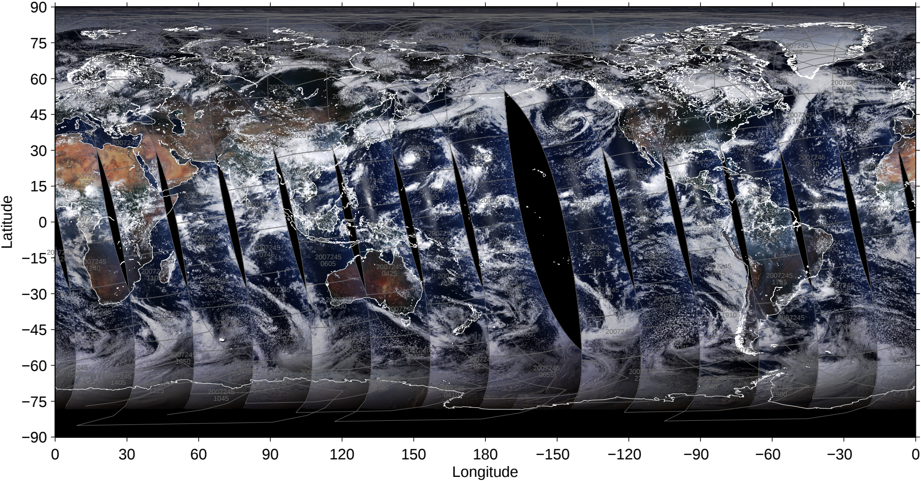
File = 200709/MYD02SSH-A2007245-pbin-005.1440-0721, RGB=645, 555, 469nm
