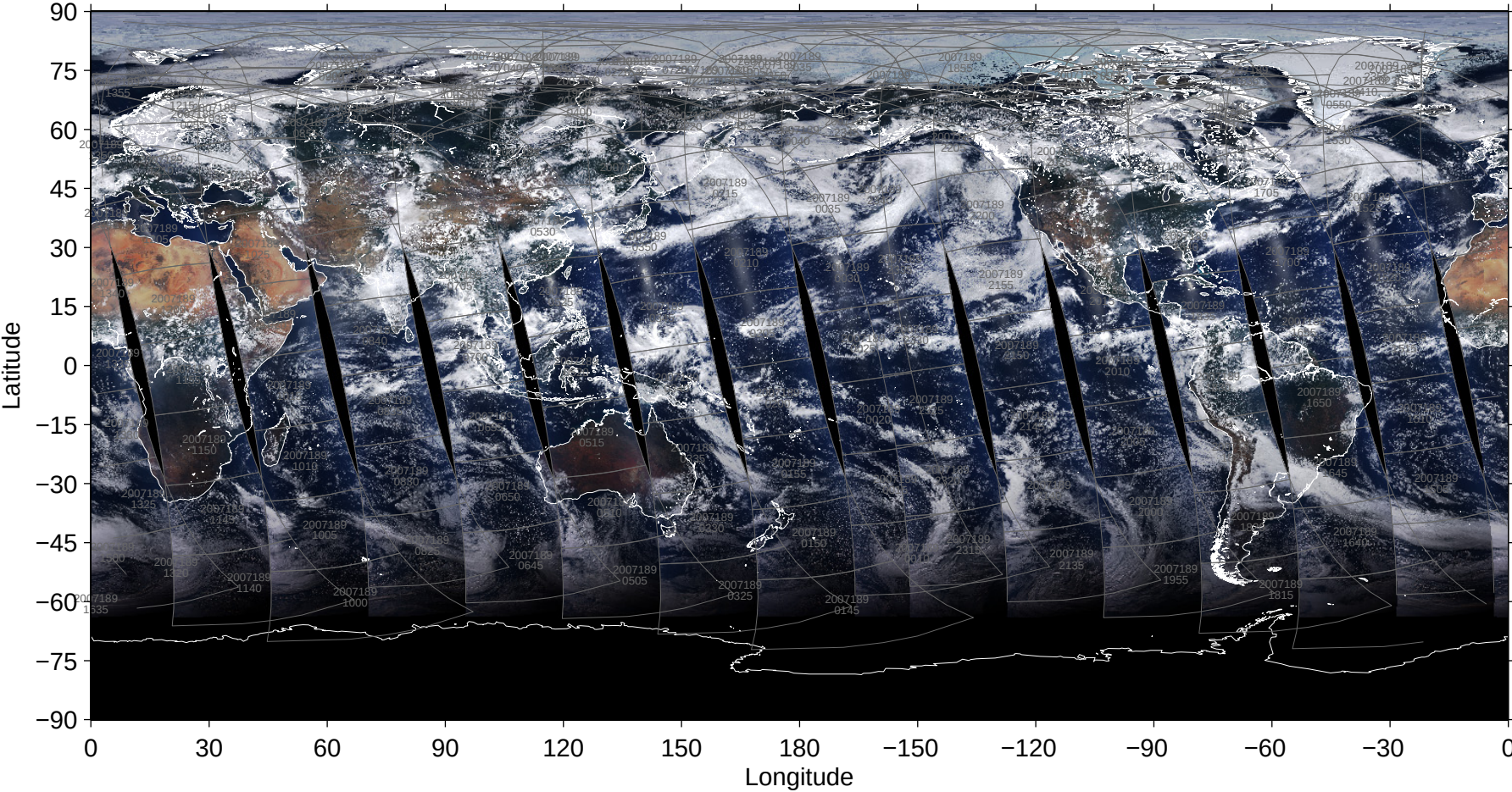
File = 200707/MYD02SSH-A2007189-pbin-005.1440-0721, RGB=645, 555, 469nm
