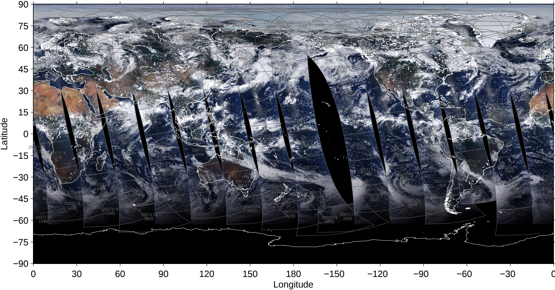
File = 200706/MYD02SSH-A2007174-pbin-005.1440-0721, RGB=645, 555, 469nm
