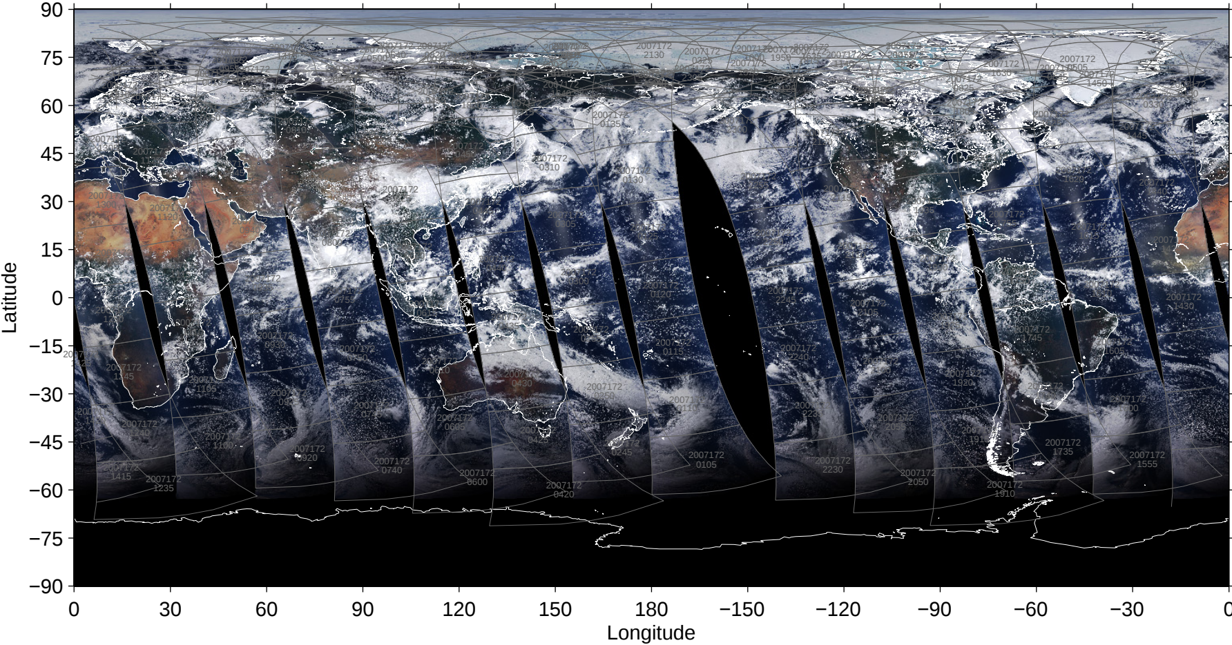
File = 200706/MYD02SSH-A2007172-pbin-005.1440-0721, RGB=645, 555, 469nm
