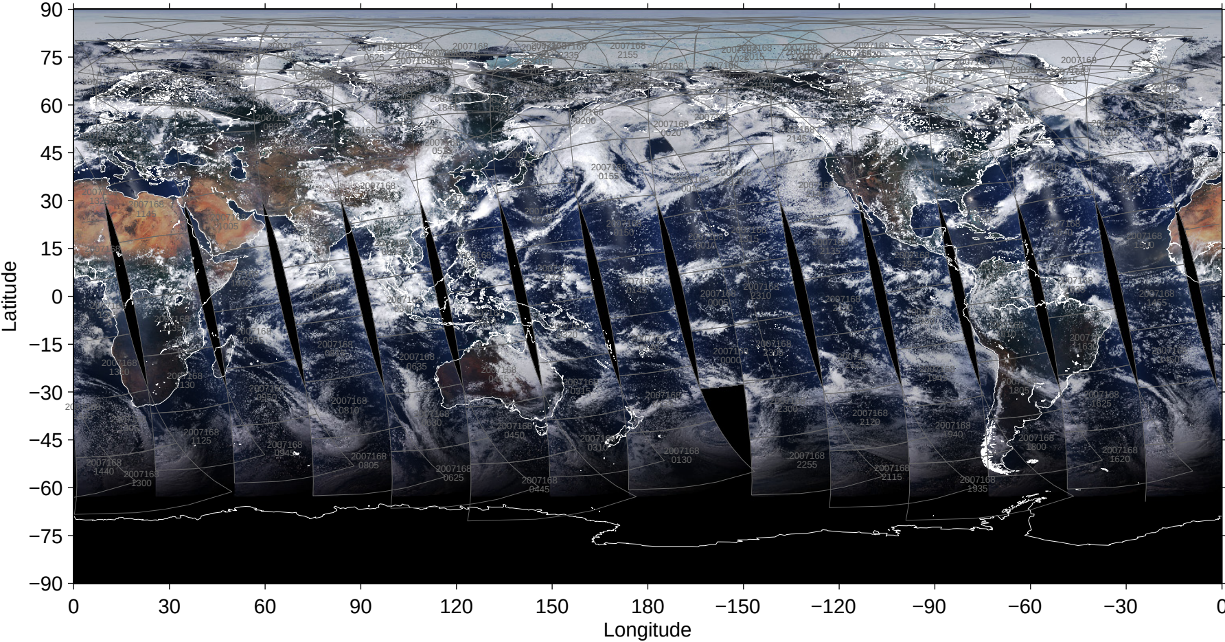
File = 200706/MYD02SSH-A2007168-pbin-005.1440-0721, RGB=645, 555, 469nm
