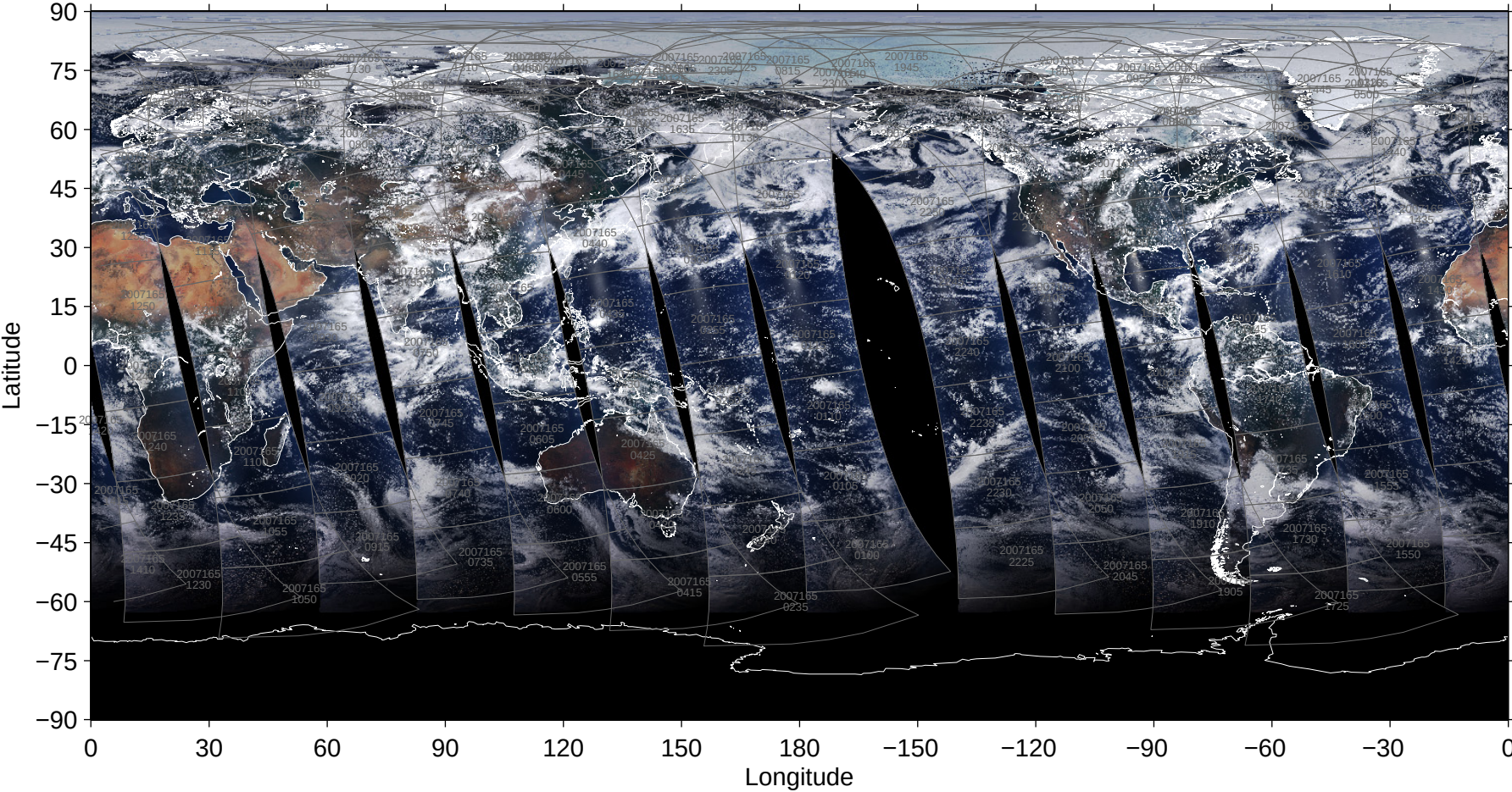
File = 200706/MYD02SSH-A2007165-pbin-005.1440-0721, RGB=645, 555, 469nm
