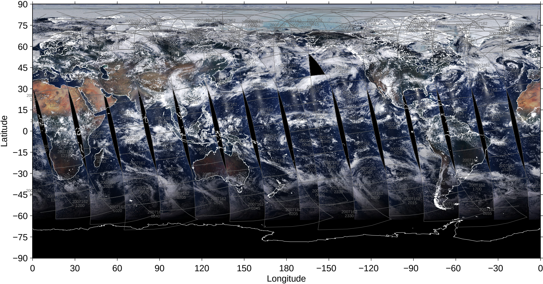
File = 200706/MYD02SSH-A2007162-pbin-005.1440-0721, RGB=645, 555, 469nm
