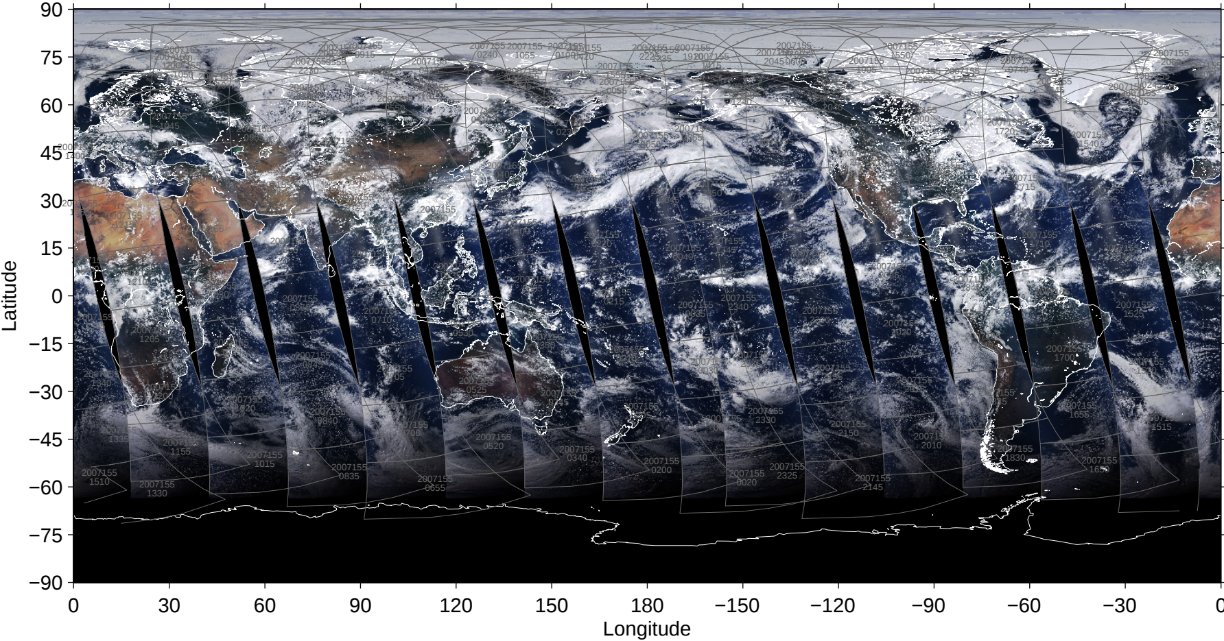
File = 200706/MYD02SSH-A2007155-pbin-005.1440-0721, RGB=645, 555, 469nm
