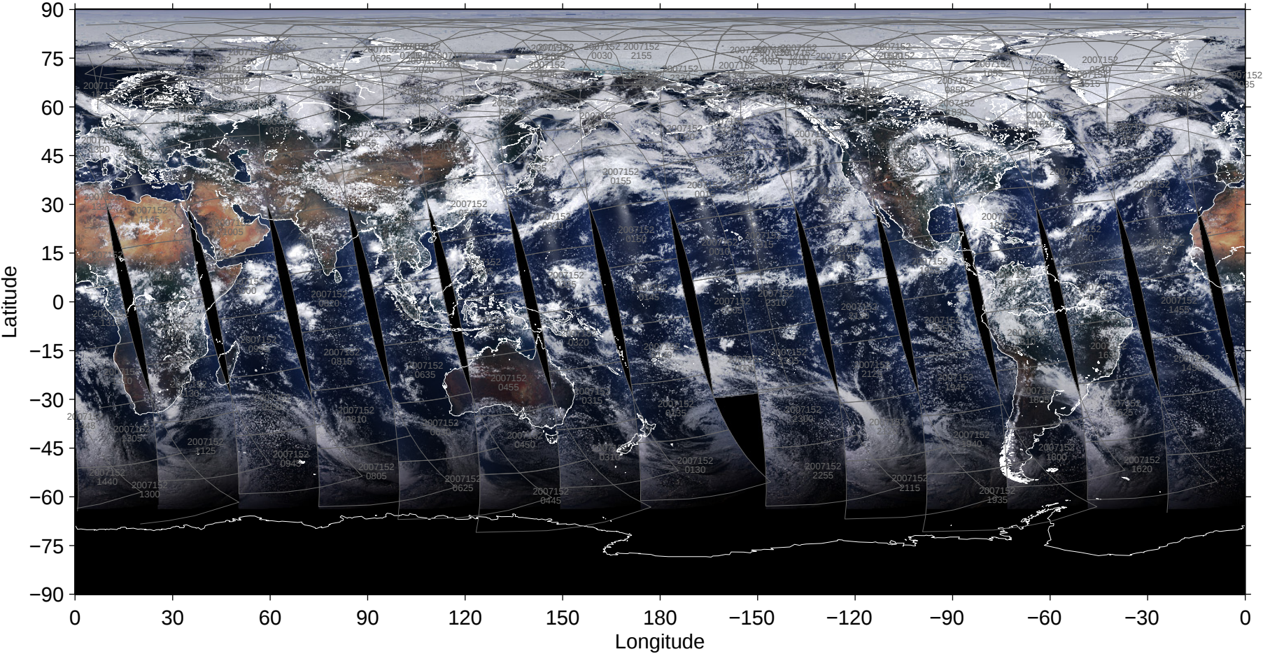
File = 200706/MYD02SSH-A2007152-pbin-005.1440-0721, RGB=645, 555, 469nm
