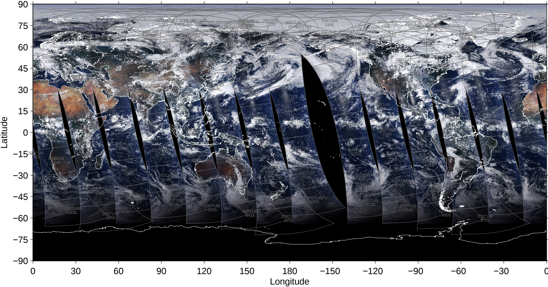
File = 200705/MYD02SSH-A2007149-pbin-005.1440-0721, RGB=645, 555, 469nm
