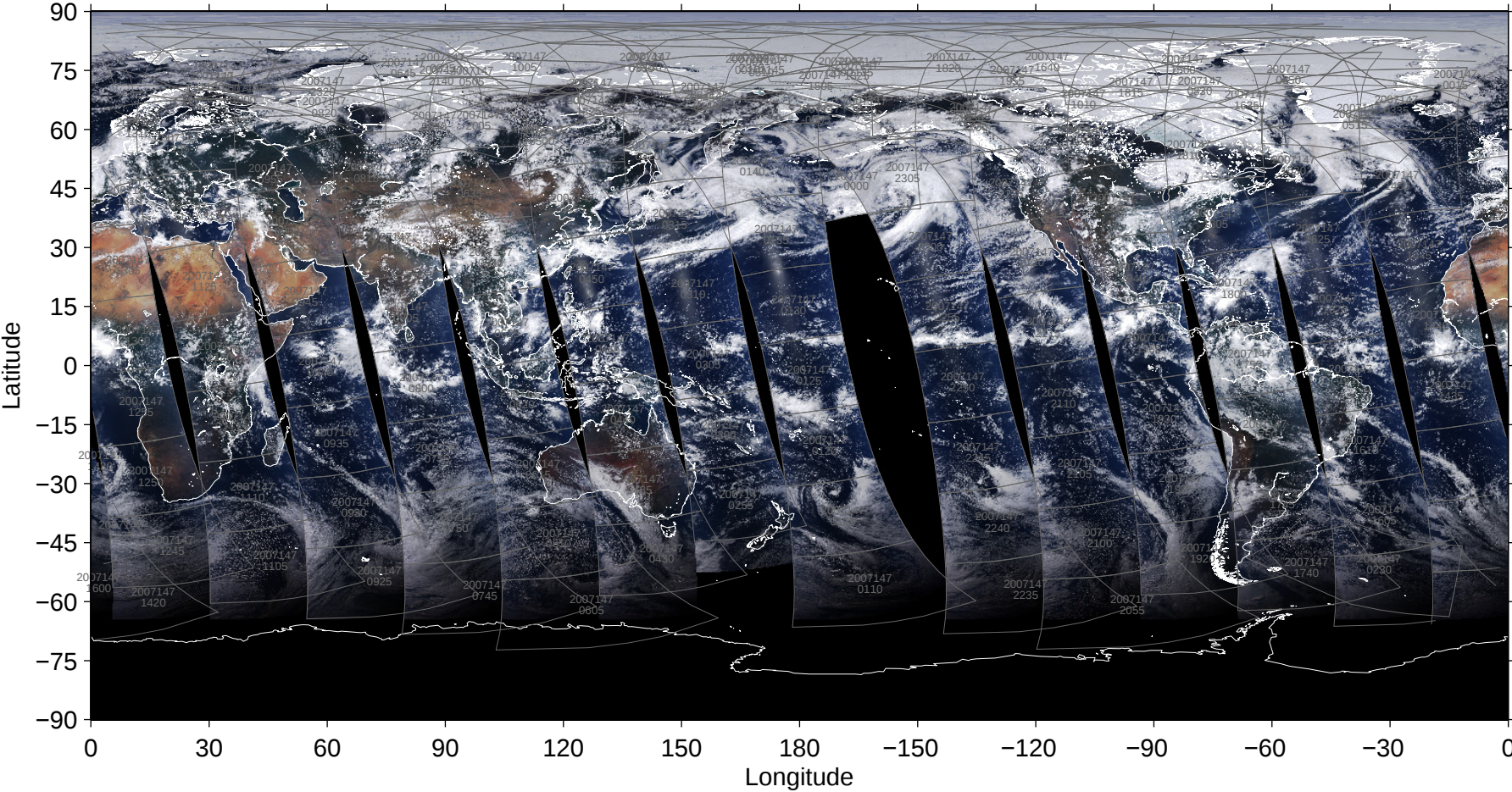
File = 200705/MYD02SSH-A2007147-pbin-005.1440-0721, RGB=645, 555, 469nm
