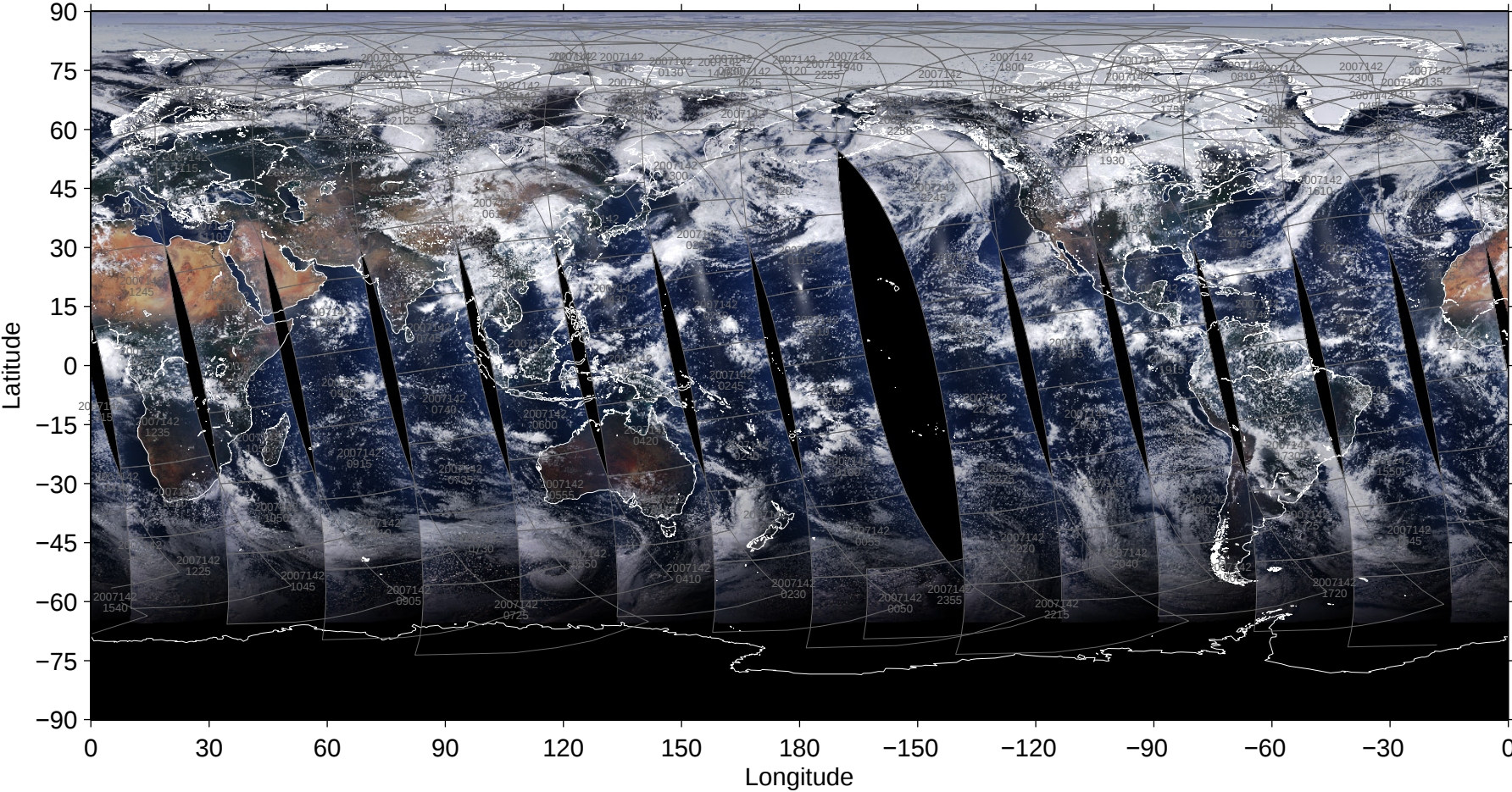
File = 200705/MYD02SSH-A2007142-pbin-005.1440-0721, RGB=645, 555, 469nm
