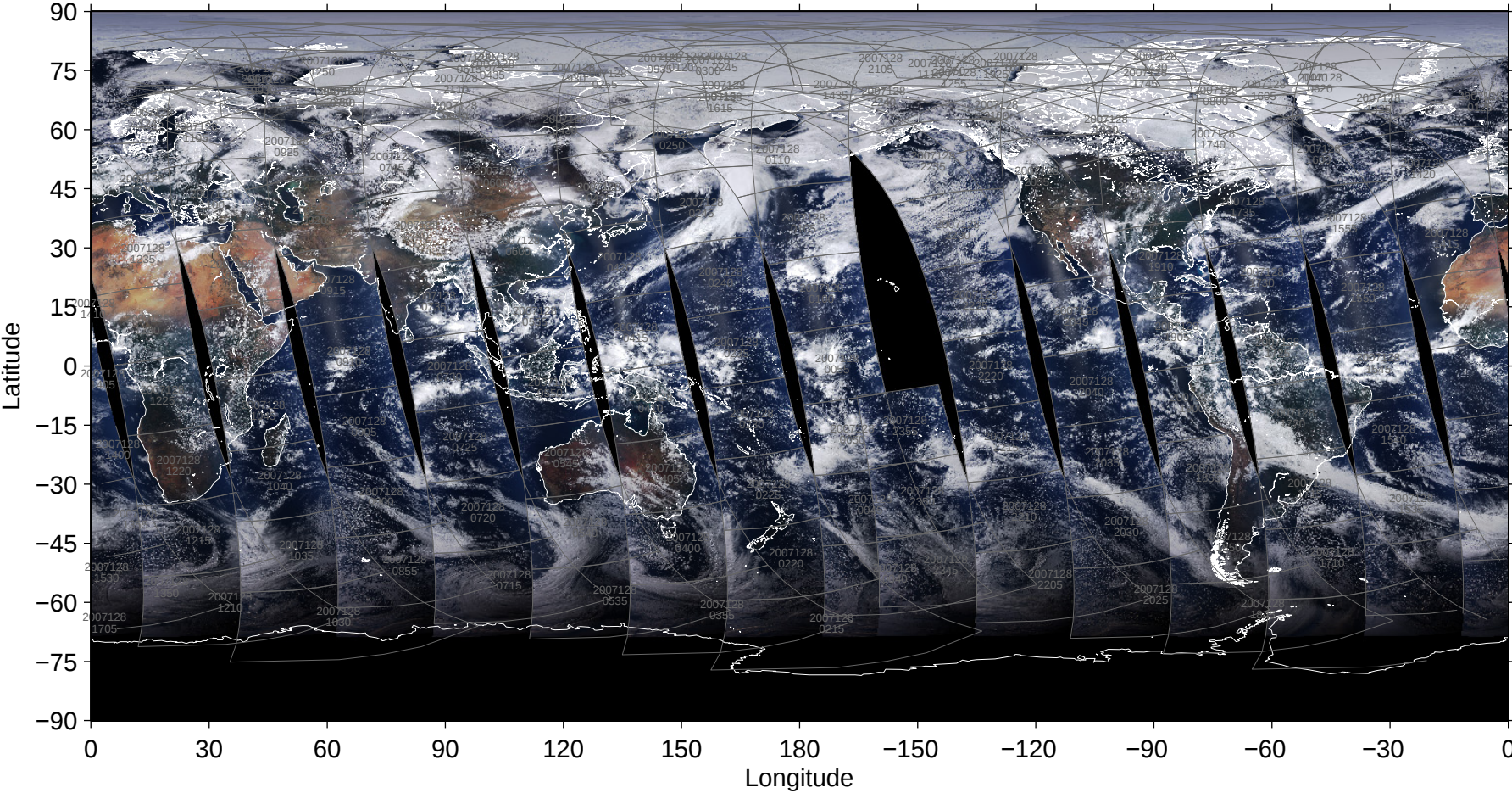
File = 200705/MYD02SSH-A2007128-pbin-005.1440-0721, RGB=645, 555, 469nm
