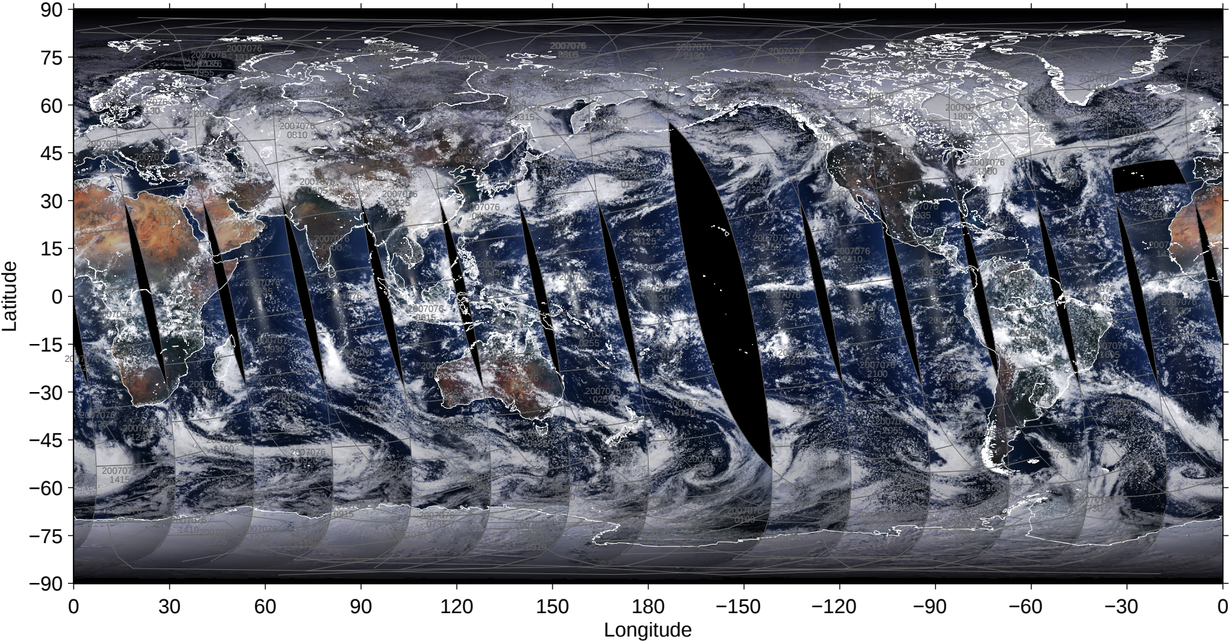
File = 200703/MYD02SSH-A2007076-pbin-005.1440-0721, RGB=645, 555, 469nm
