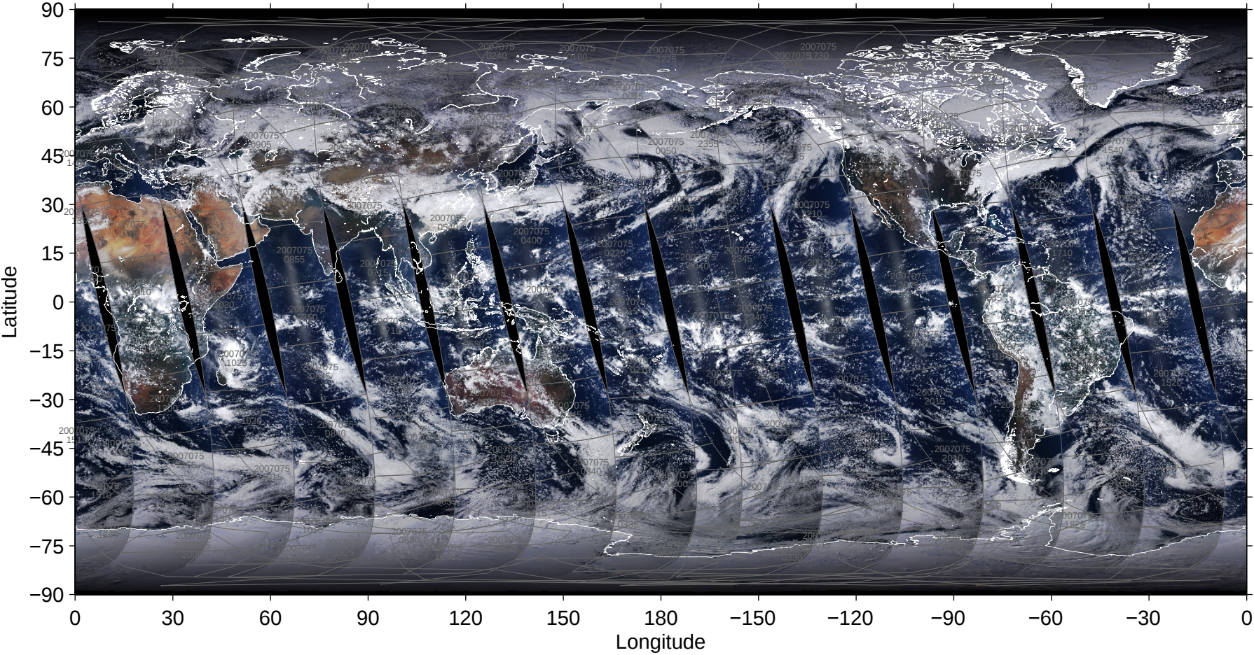
File = 200703/MYD02SSH-A2007075-pbin-005.1440-0721, RGB=645, 555, 469nm
