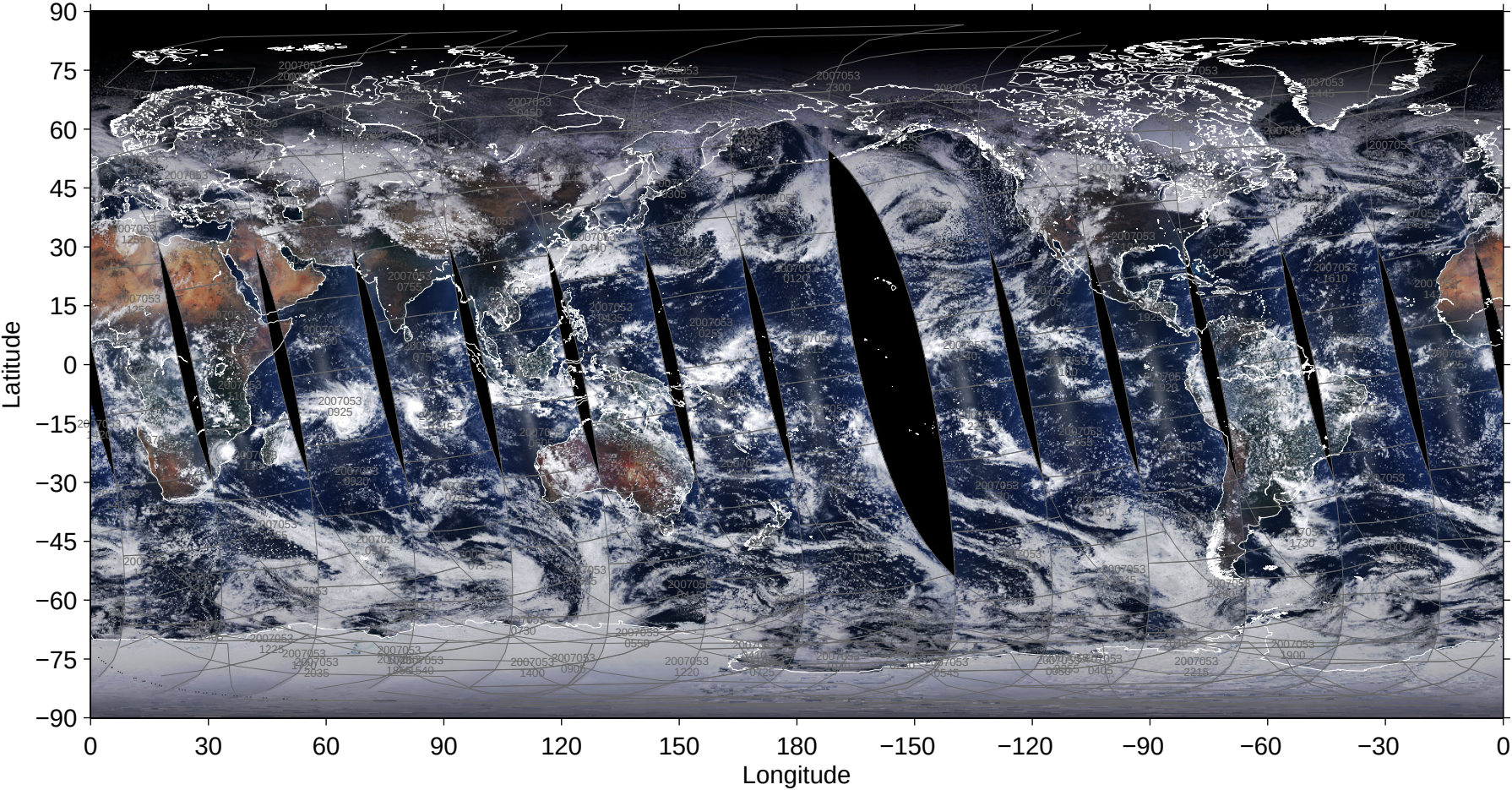
File = 200702/MYD02SSH-A2007053-pbin-005.1440-0721, RGB=645, 555, 469nm
