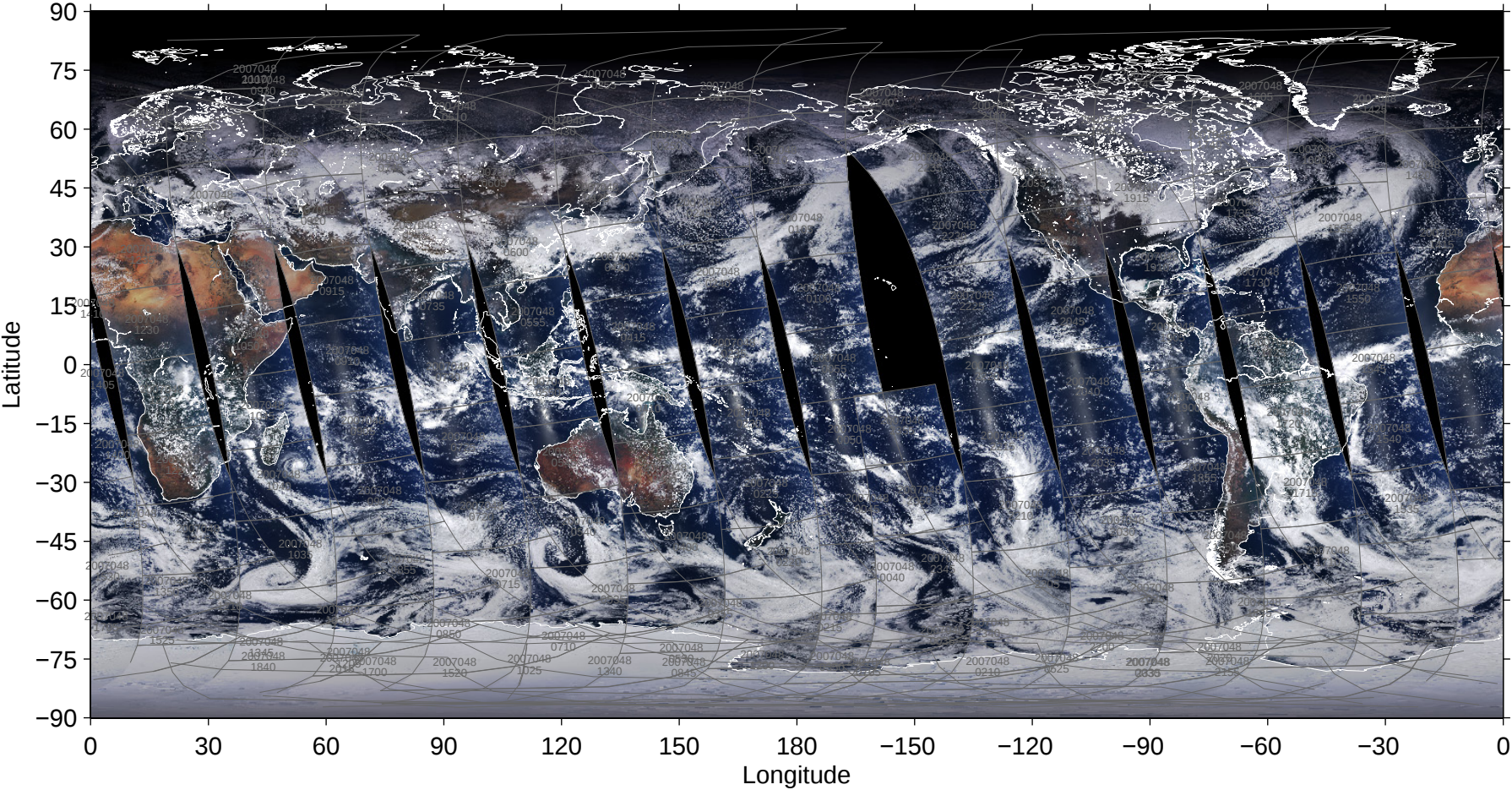
File = 200702/MYD02SSH-A2007048-pbin-005.1440-0721, RGB=645, 555, 469nm
