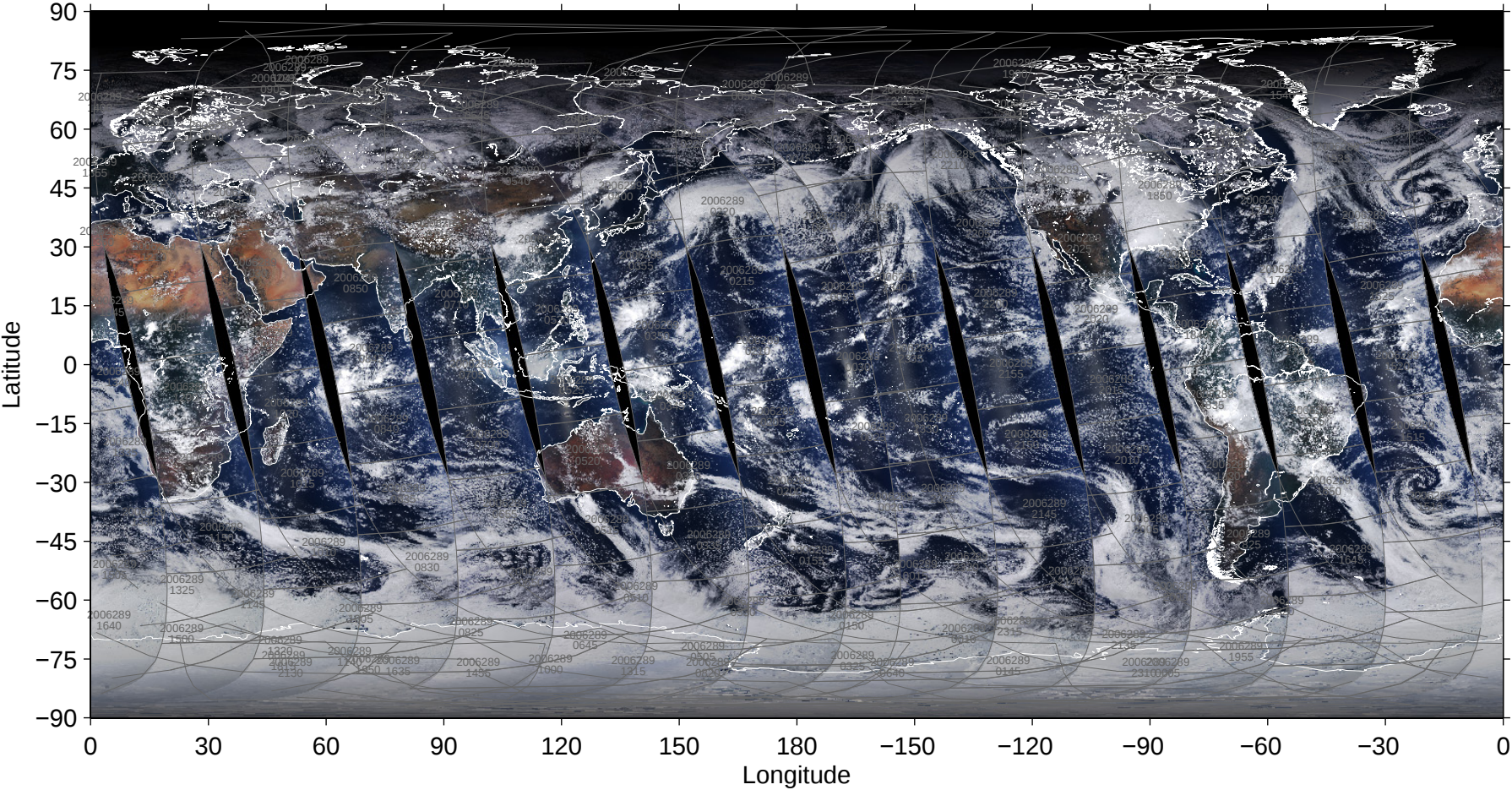
File = 200610/MYD02SSH-A2006289-pbin-005.1440-0721, RGB=645, 555, 469nm
