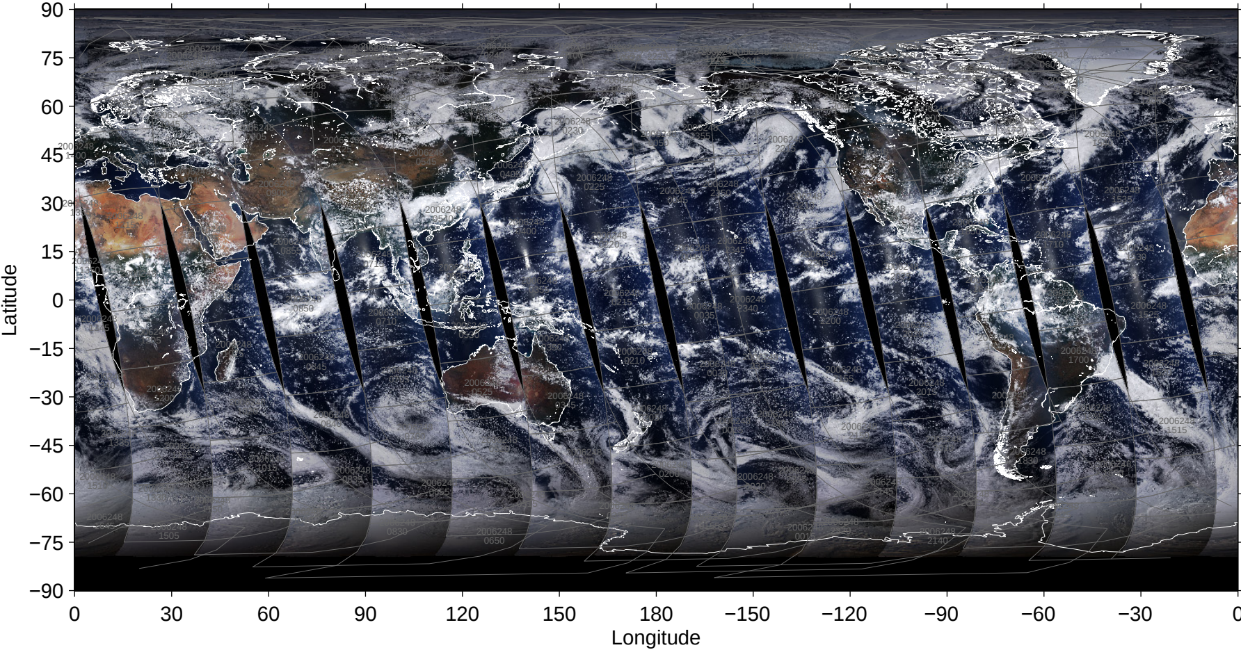
File = 200609/MYD02SSH-A2006248-pbin-005.1440-0721, RGB=645, 555, 469nm
