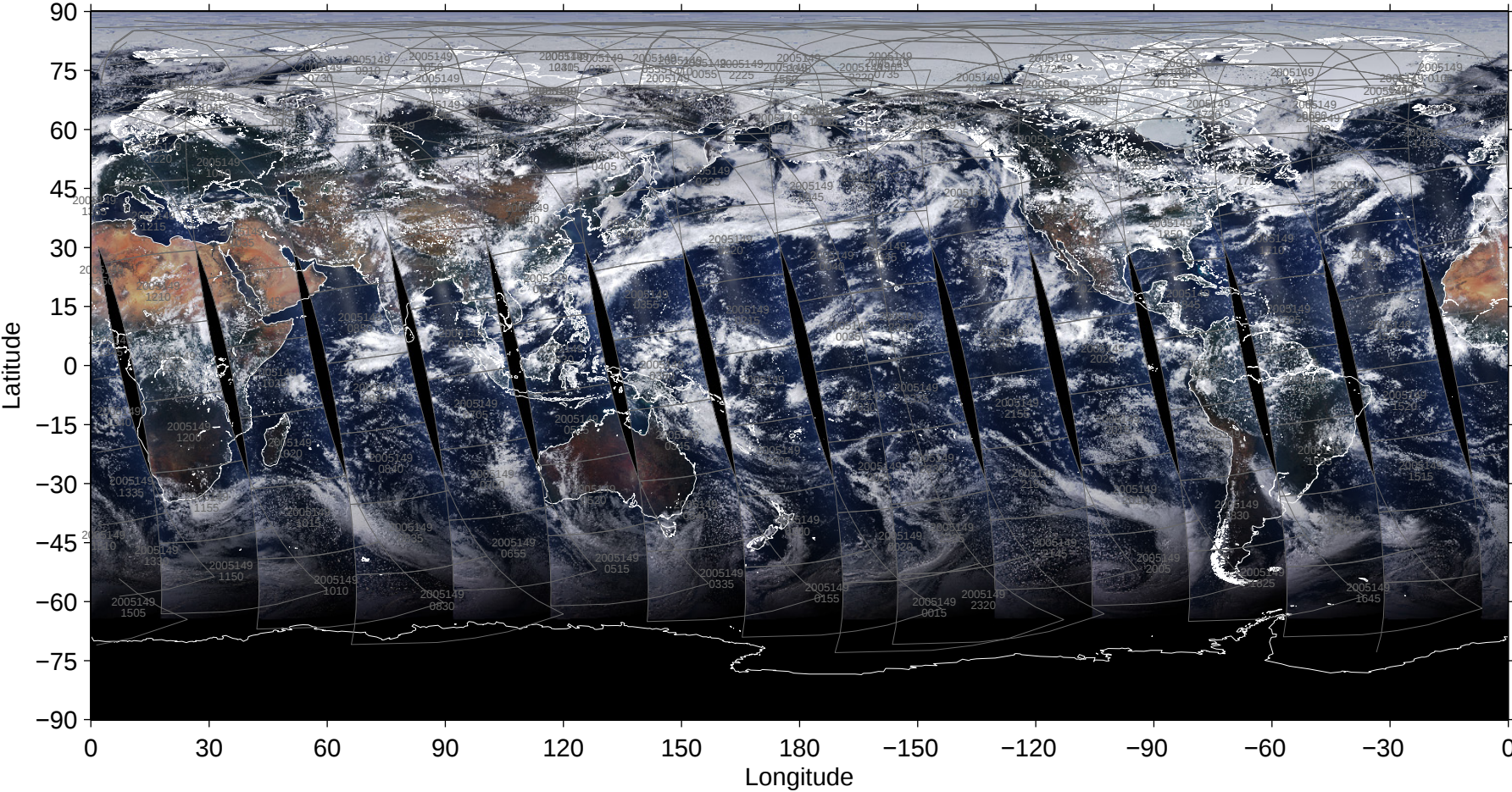
File = MYD02SSH-A2005149-pbin-005.1440-0721, RGB=645, 555, 469nm
