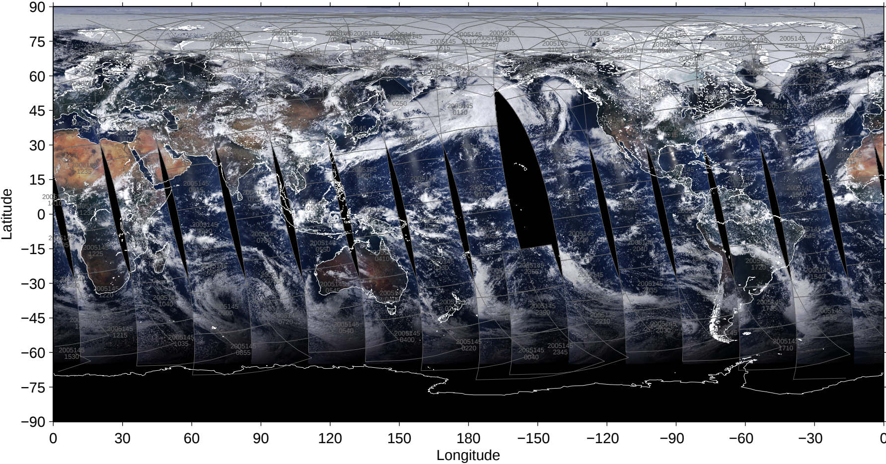
File = MYD02SSH-A2005145-pbin-005.1440-0721, RGB=645, 555, 469nm
