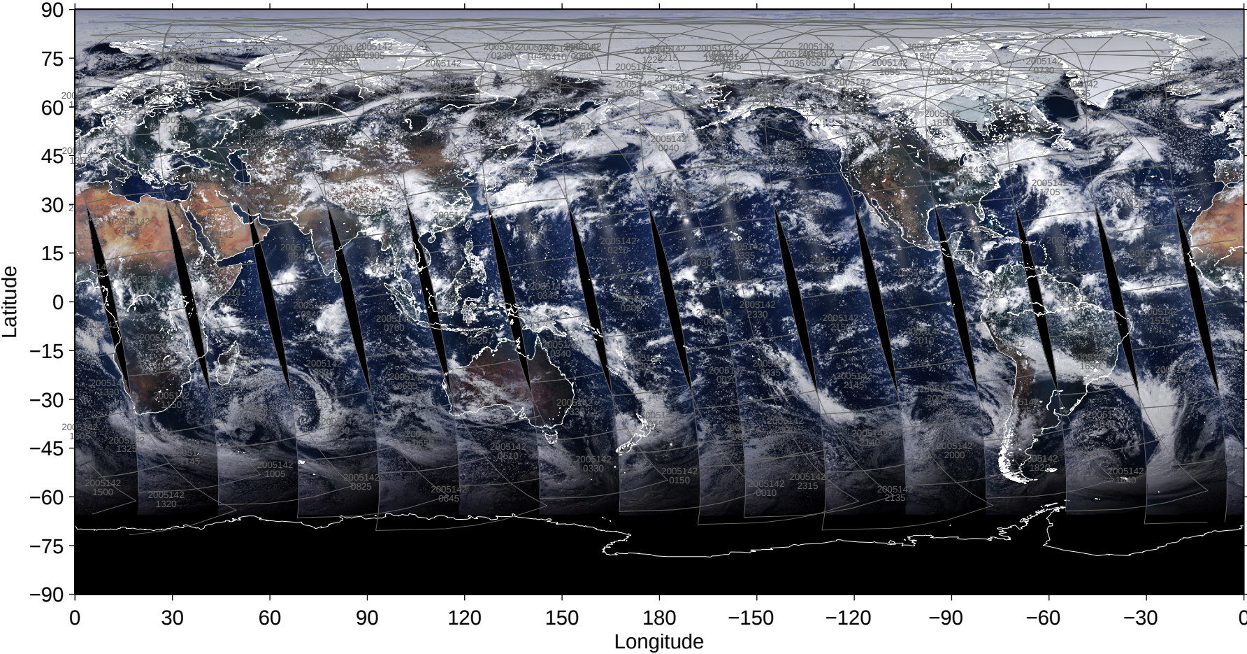
File = MYD02SSH-A2005142-pbin-005.1440-0721, RGB=645, 555, 469nm
