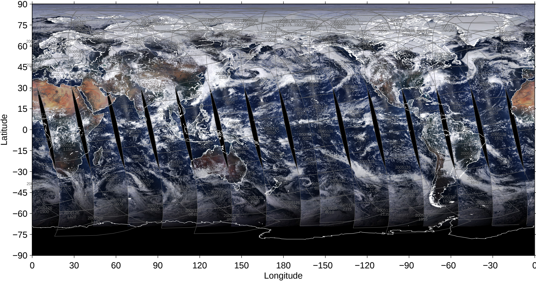
File = MYD02SSH-A2005126-pbin-005.1440-0721, RGB=645, 555, 469nm
