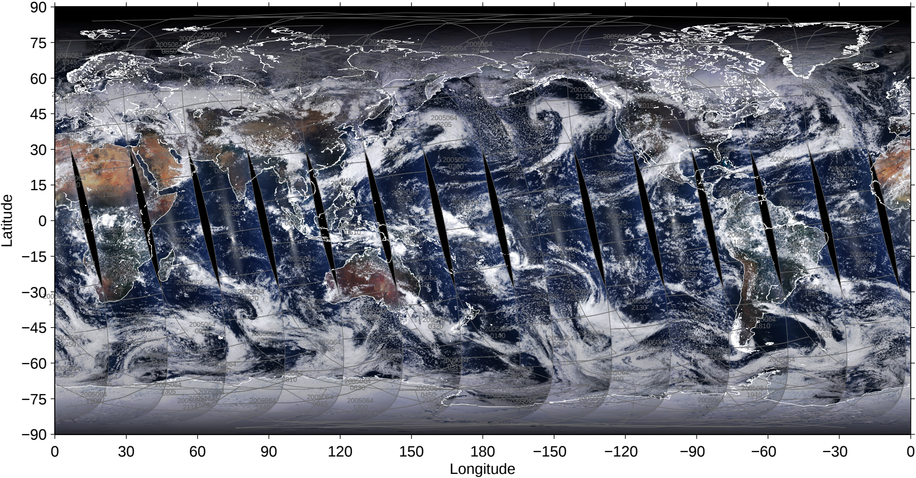
File = MYD02SSH-A2005064-pbin-005.1440-0721, RGB=645, 555, 469nm
