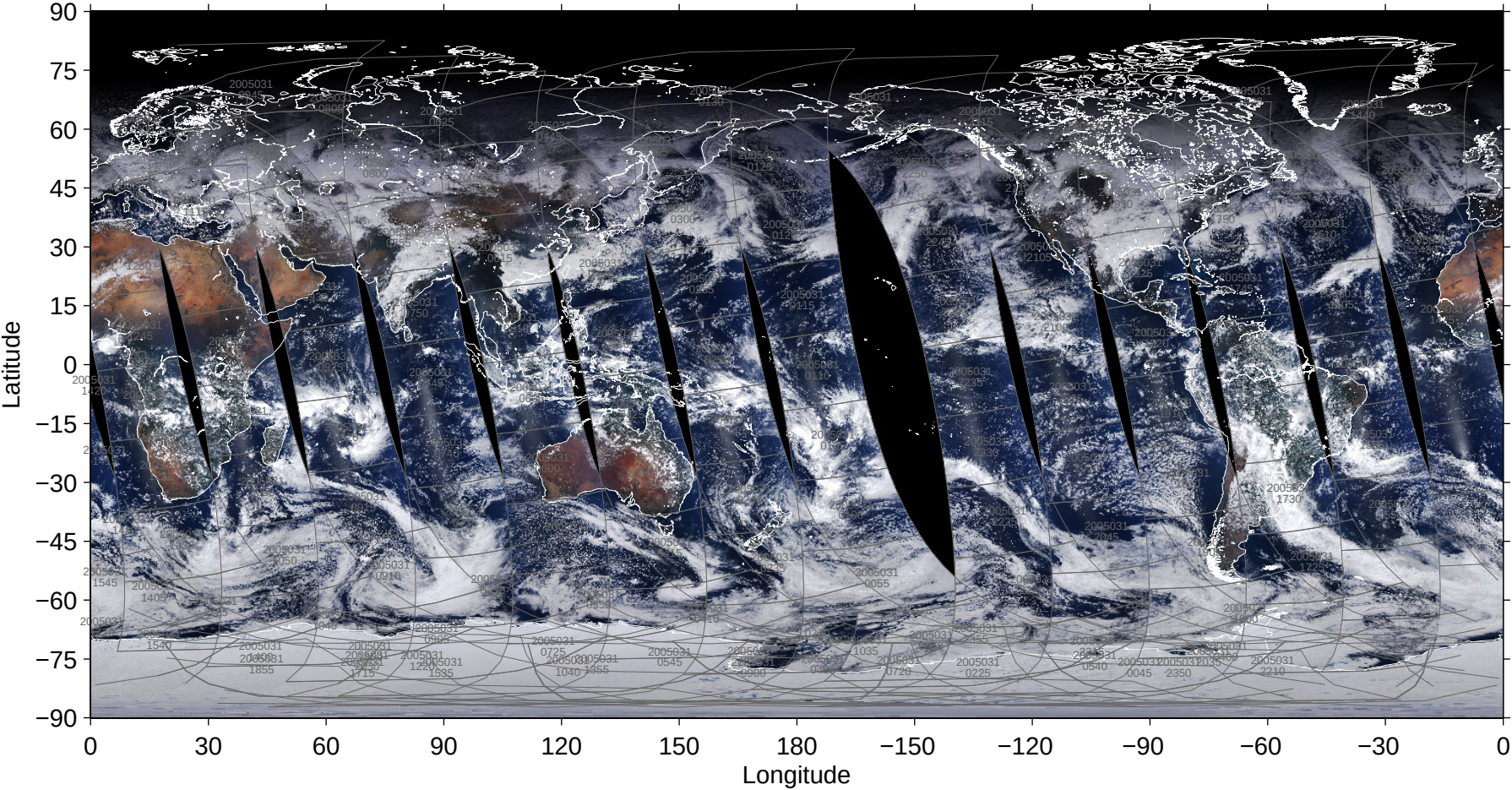
File = MYD02SSH-A2005031-pbin-005.1440-0721, RGB=645, 555, 469nm
