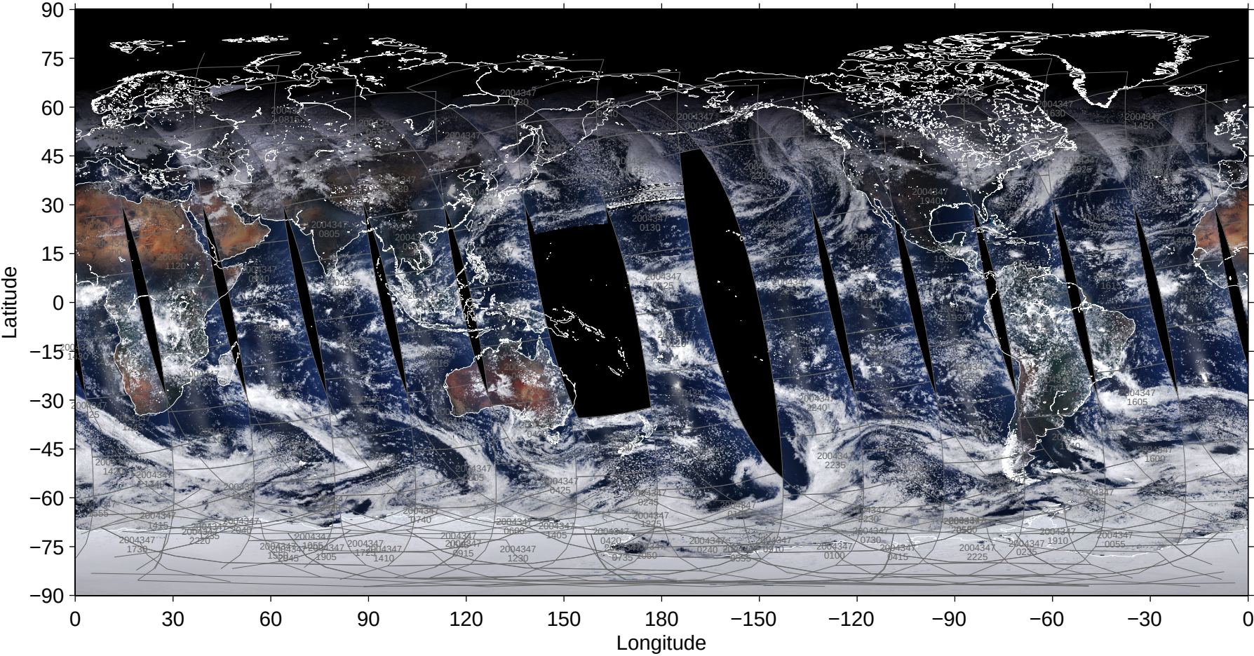
File = 200412/MYD02SSH-A2004347-pbin-004.1440-0721, RGB=645, 555, 469nm
