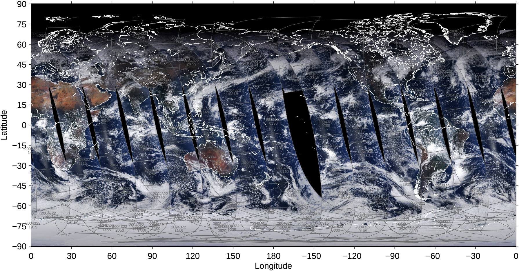
File = 200411/MYD02SSH-A2004322-pbin-004.1440-0721, RGB=645, 555, 469nm
