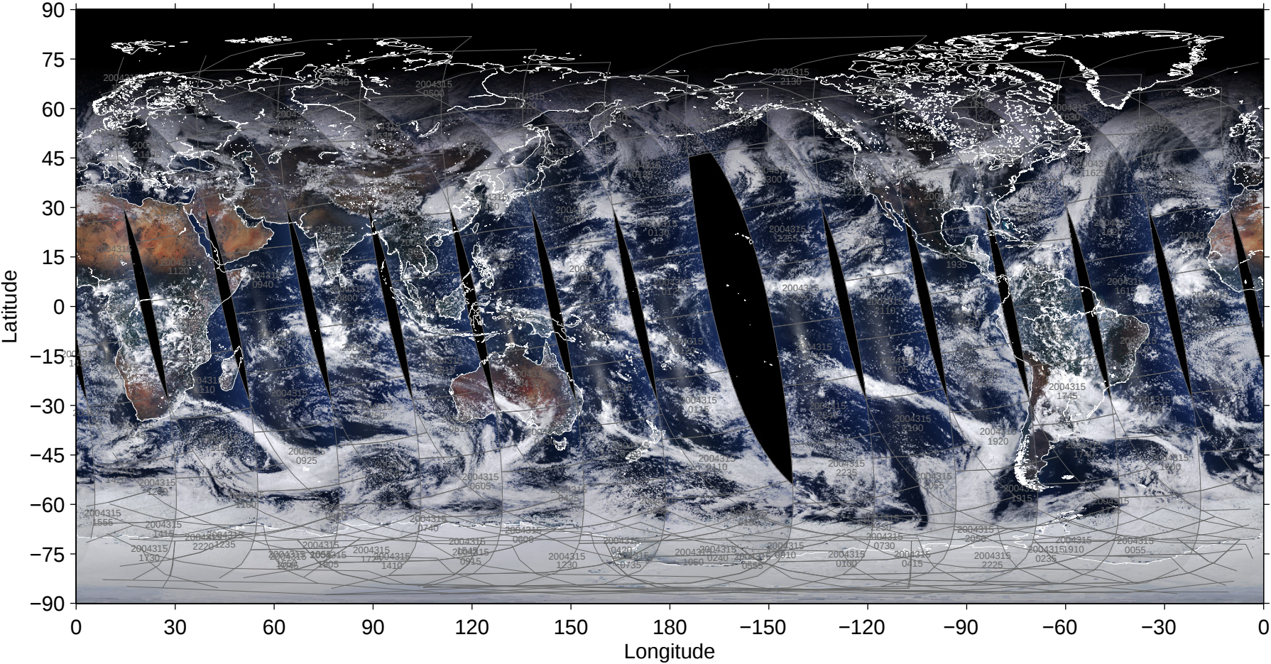
File = 200411/MYD02SSH-A2004315-pbin-004.1440-0721, RGB=645, 555, 469nm
