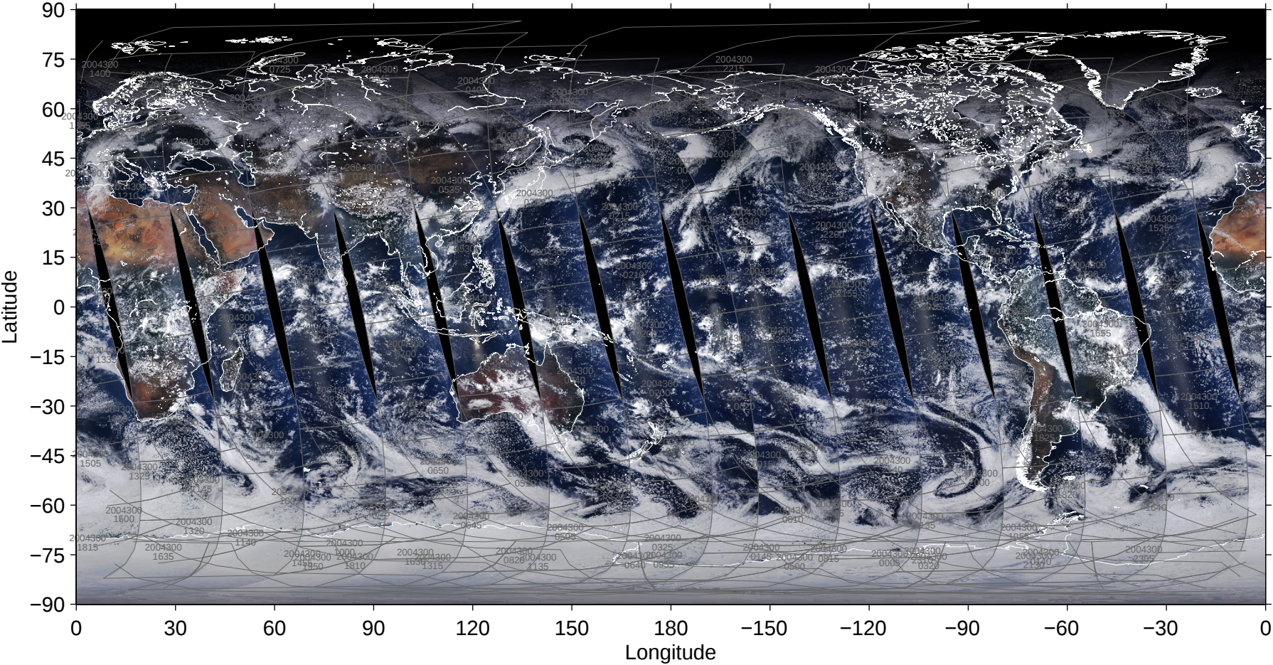
File = 200410/MYD02SSH-A2004300-pbin-004.1440-0721, RGB=645, 555, 469nm
