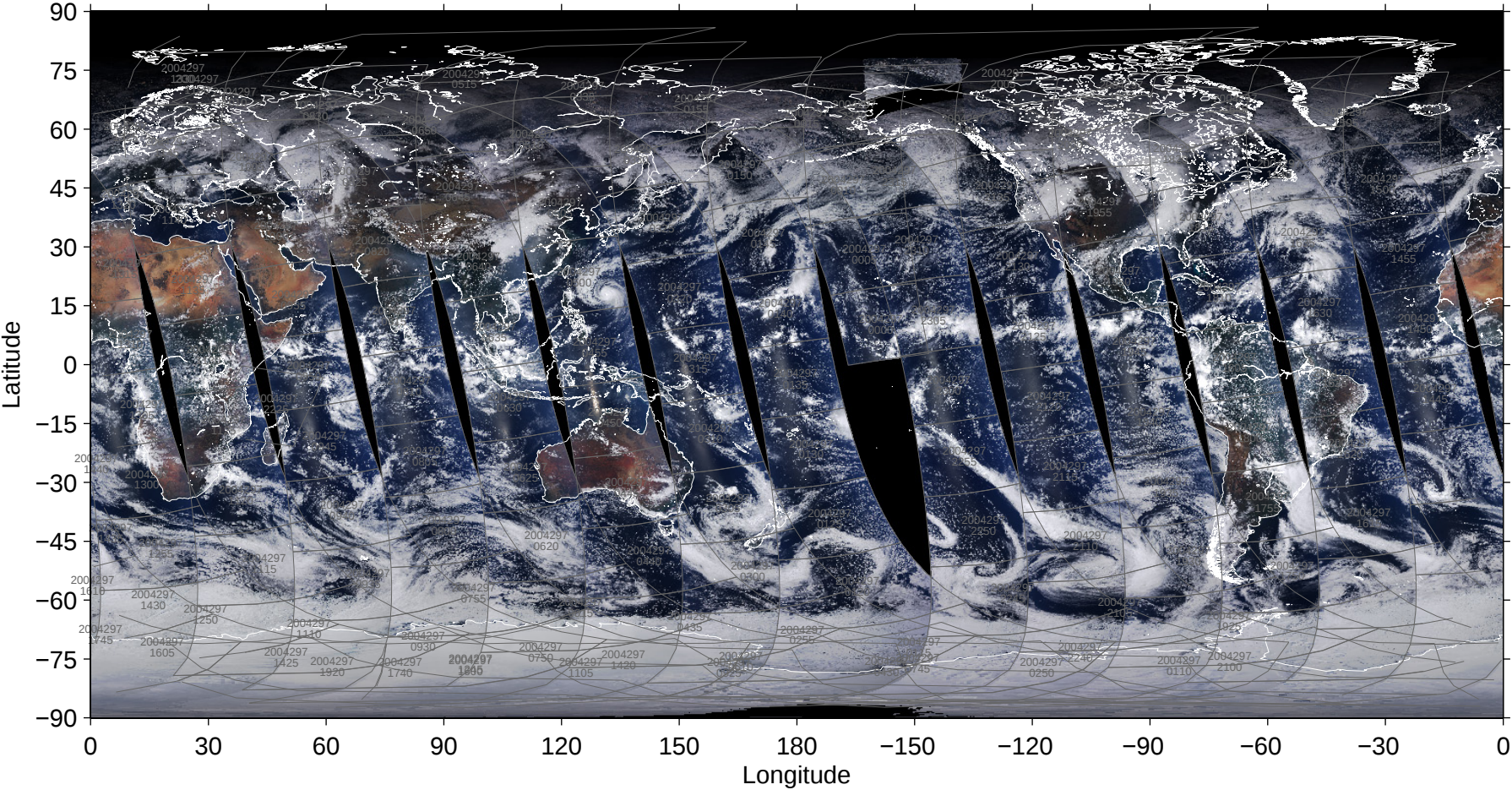
File = 200410/MYD02SSH-A2004297-pbin-004.1440-0721, RGB=645, 555, 469nm
