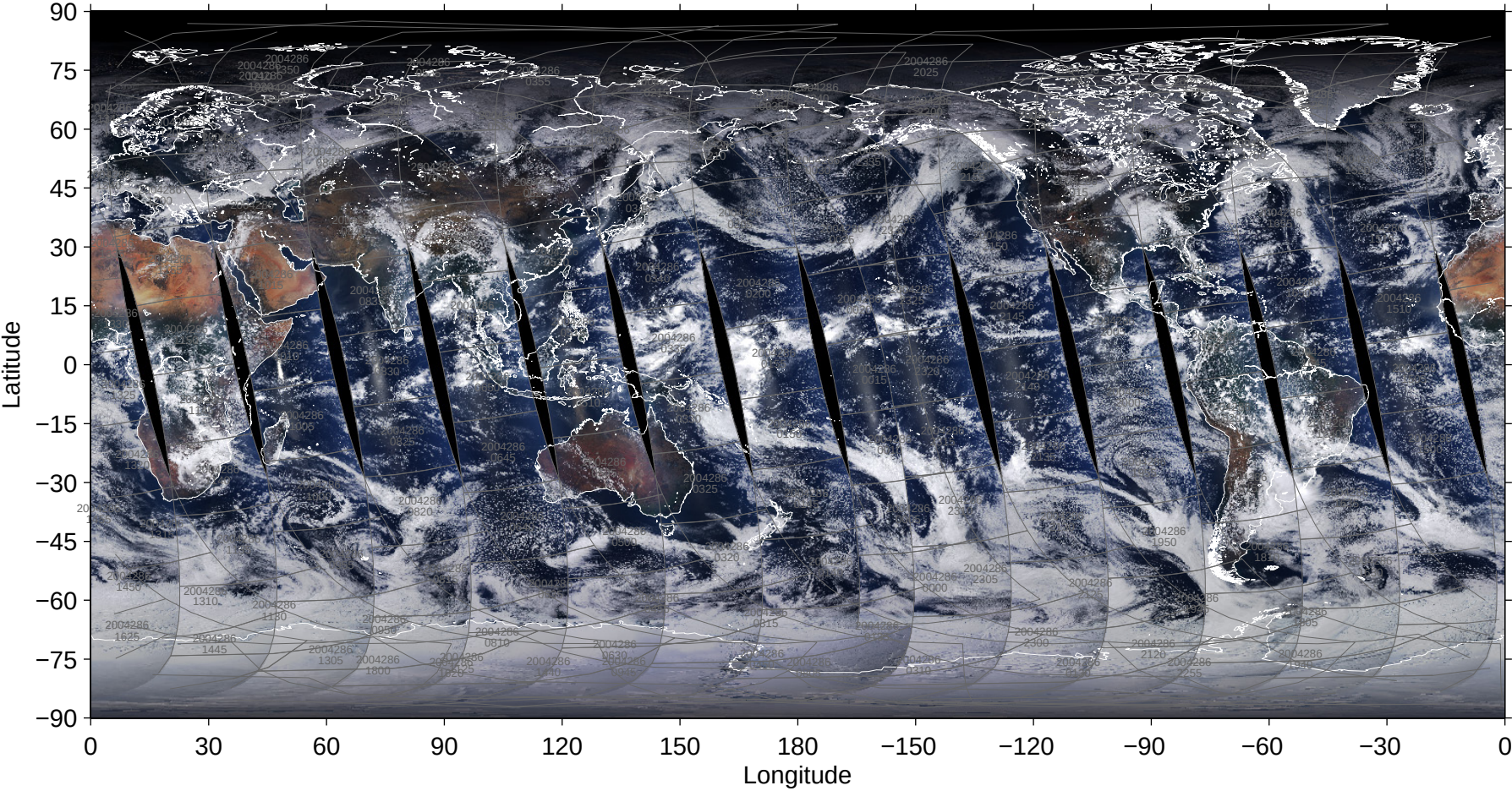
File = 200410/MYD02SSH-A2004286-pbin-004.1440-0721, RGB=645, 555, 469nm
