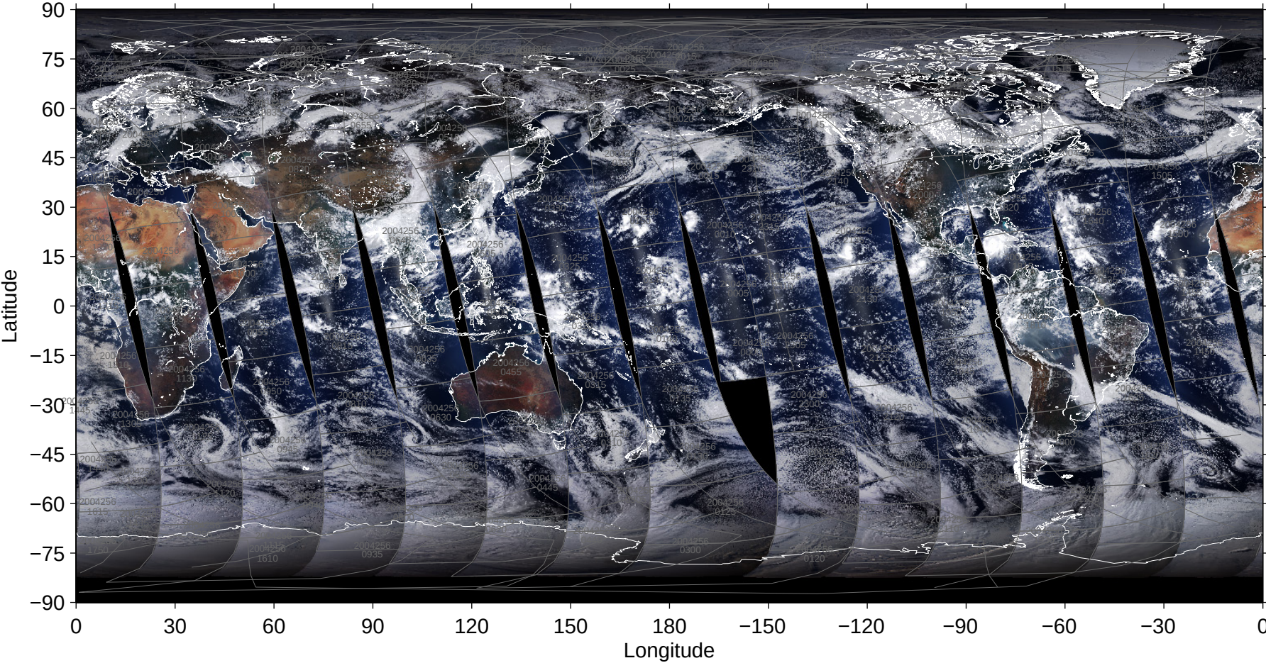
File = 200409/MYD02SSH-A2004256-pbin-004.1440-0721, RGB=645, 555, 469nm
