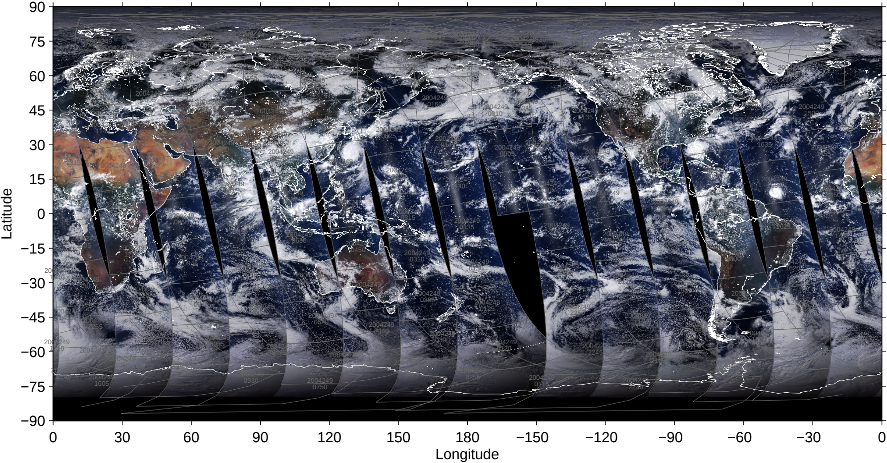
File = 200409/MYD02SSH-A2004249-pbin-004.1440-0721, RGB=645, 555, 469nm
