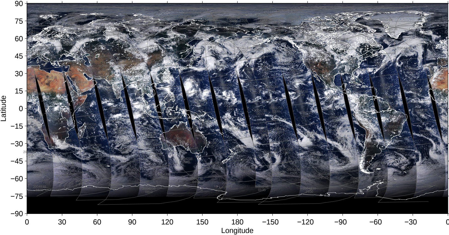
File = 200408/MYD02SSH-A2004238-pbin-004.1440-0721, RGB=645, 555, 469nm
