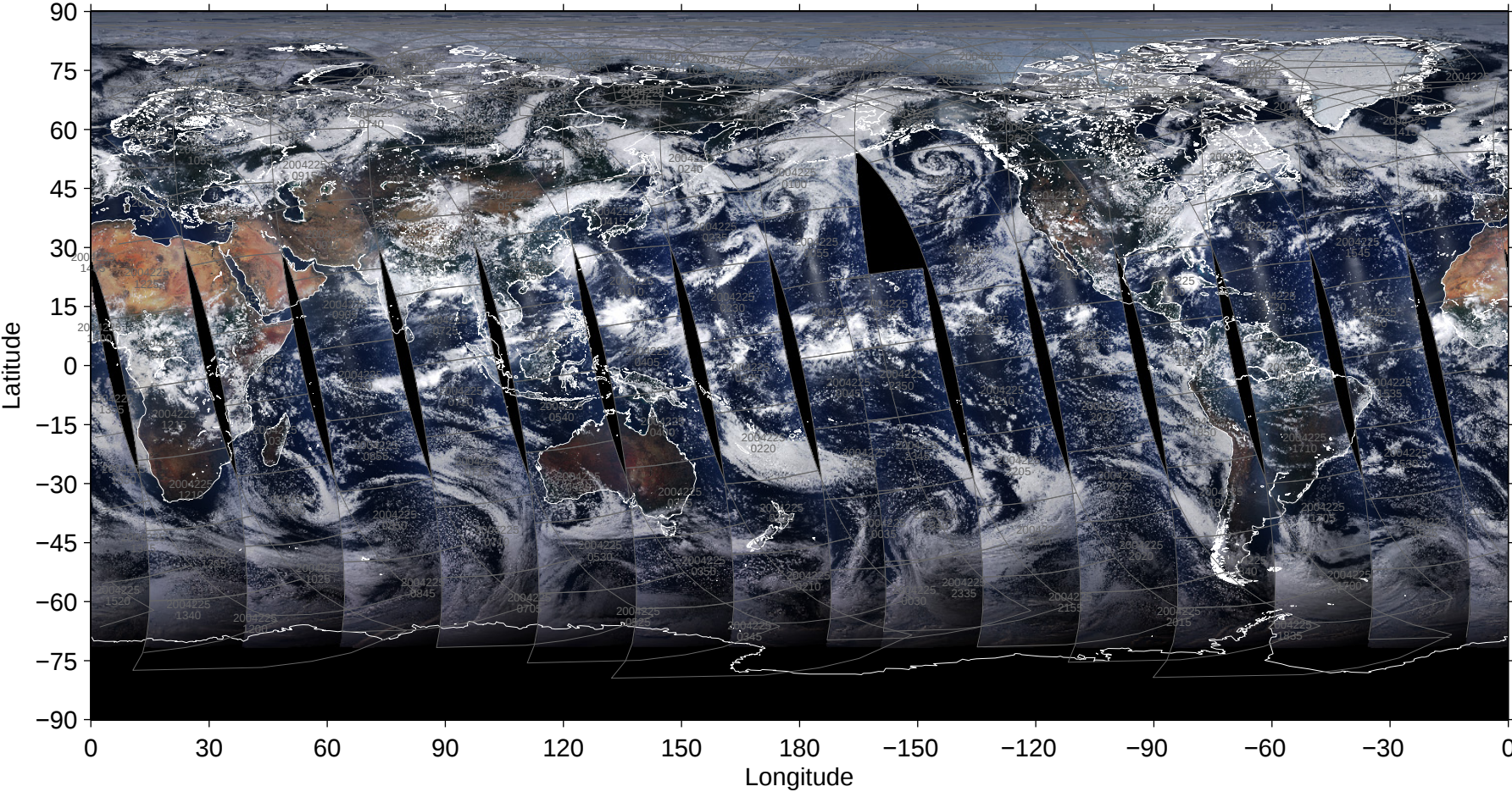
File = 200408/MYD02SSH-A2004225-pbin-004.1440-0721, RGB=645, 555, 469nm
