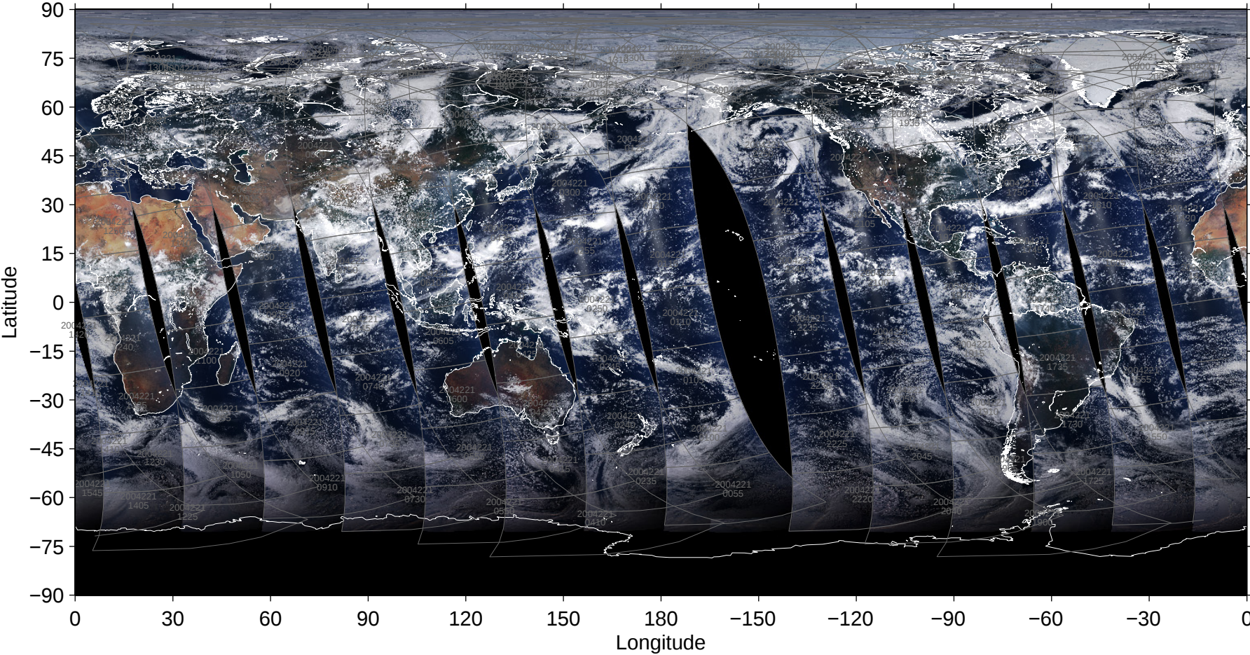
File = 200408/MYD02SSH-A2004221-pbin-004.1440-0721, RGB=645, 555, 469nm
