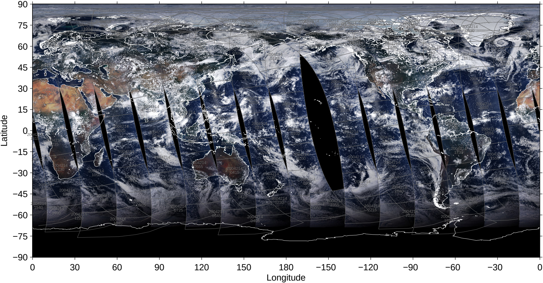
File = 200408/MYD02SSH-A2004214-pbin-004.1440-0721, RGB=645, 555, 469nm
