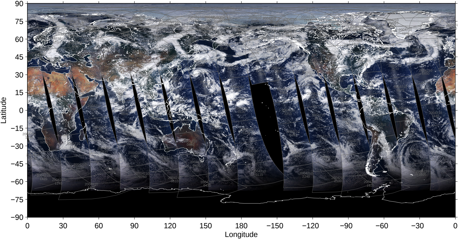
File = 200407/MYD02SSH-A2004210-pbin-004.1440-0721, RGB=645, 555, 469nm
