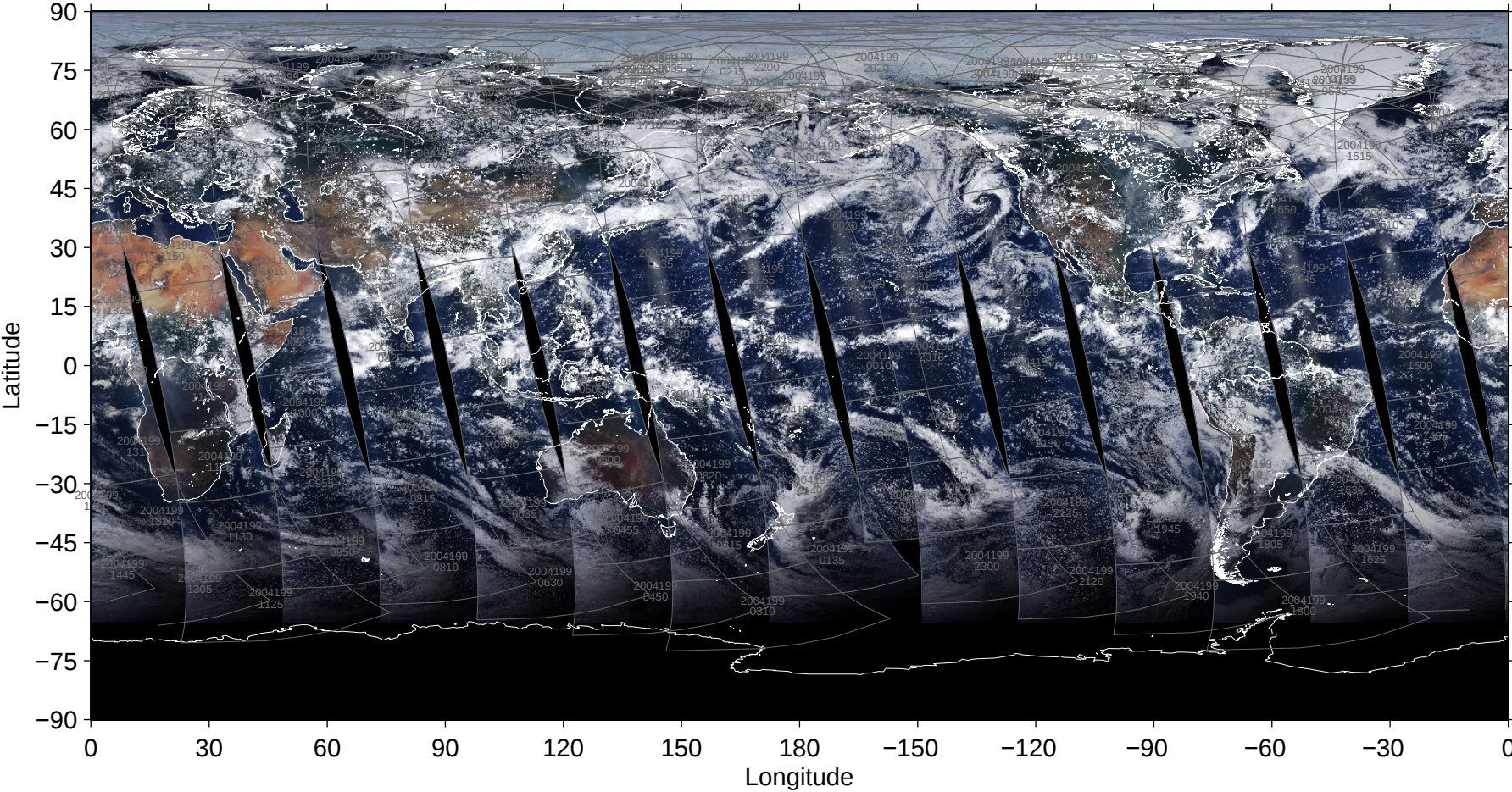
File = 200407/MYD02SSH-A2004199-pbin-004.1440-0721, RGB=645, 555, 469nm
