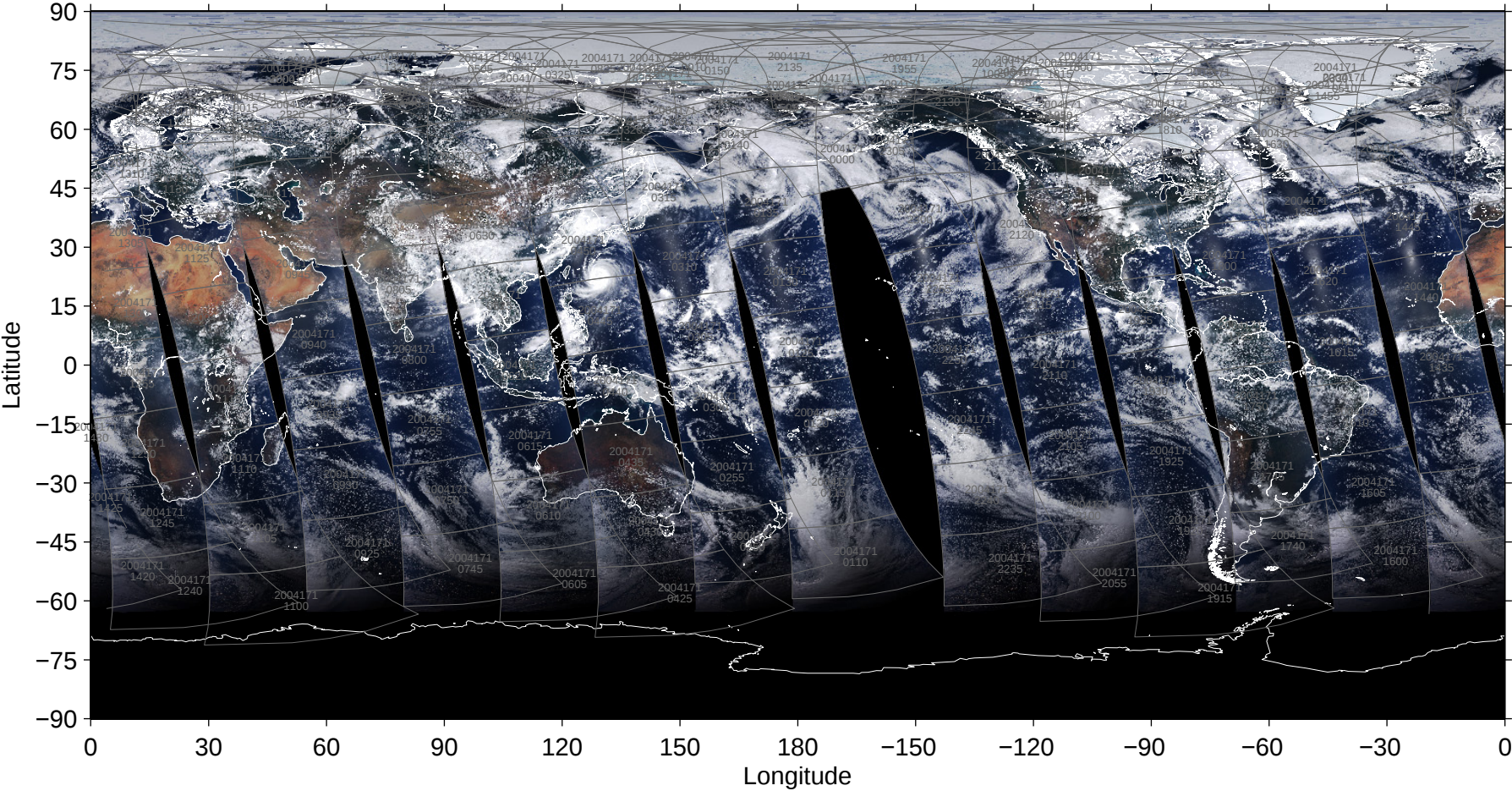
File = 200406/MYD02SSH-A2004171-pbin-005.1440-0721, RGB=645, 555, 469nm
