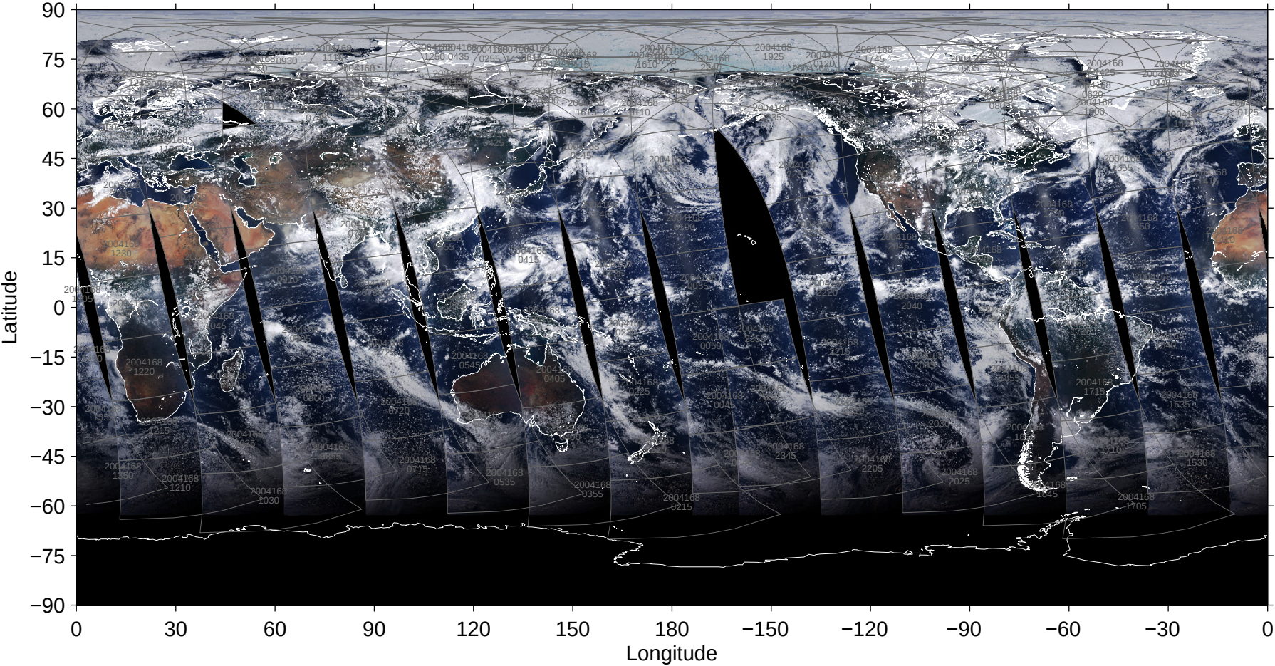
File = 200406/MYD02SSH-A2004168-pbin-005.1440-0721, RGB=645, 555, 469nm
