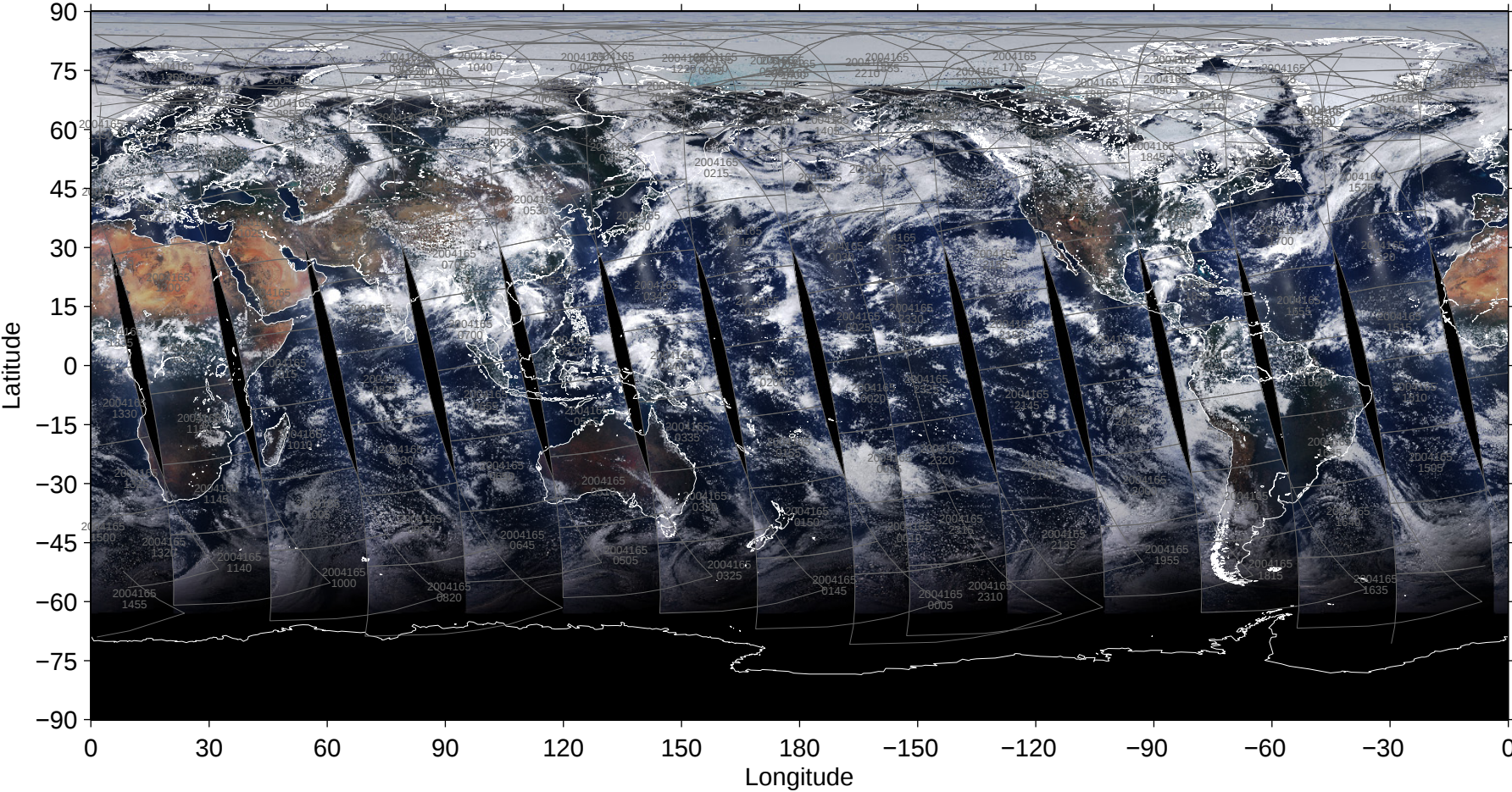
File = 200406/MYD02SSH-A2004165-pbin-005.1440-0721, RGB=645, 555, 469nm
