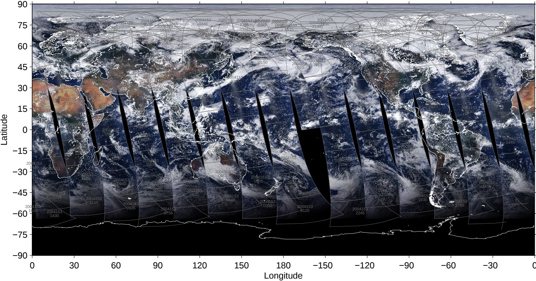
File = 200406/MYD02SSH-A2004153-pbin-005.1440-0721, RGB=645, 555, 469nm
