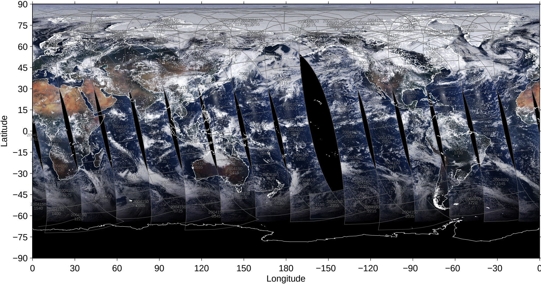
File = 200405/MYD02SSH-A2004150-pbin-005.1440-0721, RGB=645, 555, 469nm
