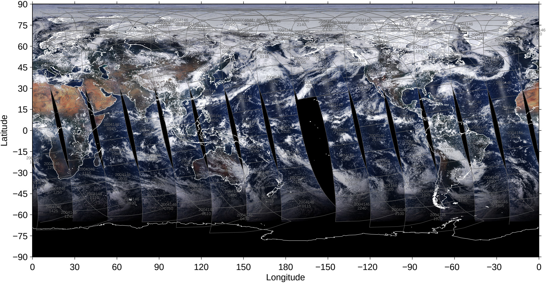
File = 200405/MYD02SSH-A2004146-pbin-005.1440-0721, RGB=645, 555, 469nm
